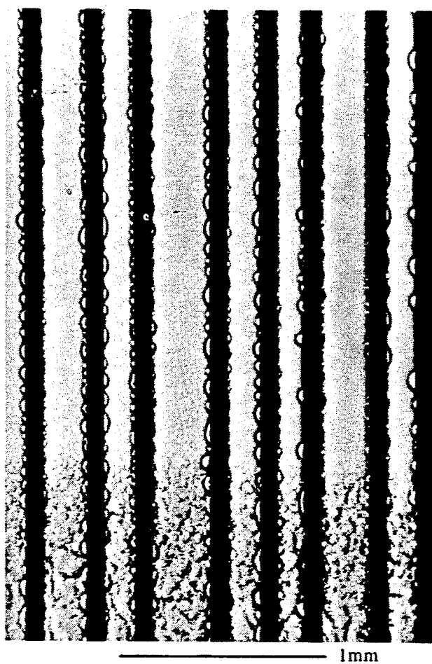
Succinonitrile-10wt. pct Glycerine Growth Velocity = 0.6\mu\text{m/s} Temperature Gradient = 45\text{K/cm} Enamel-Coated Copper Fibers
