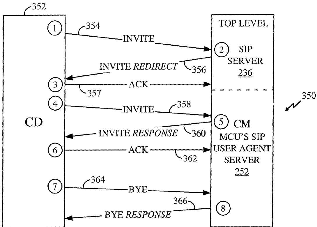
FIG. 11 SIP CALL SIGNALING
