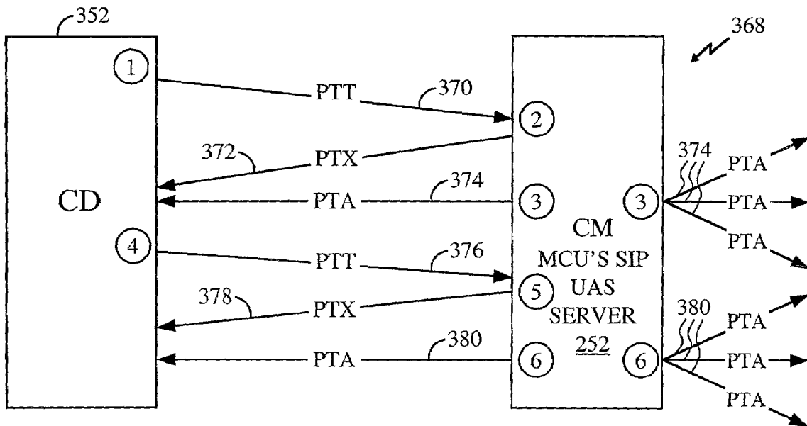
FIG. 12 MEDIA SIGNALING MESSAGE SEQUENCE (PTT)
