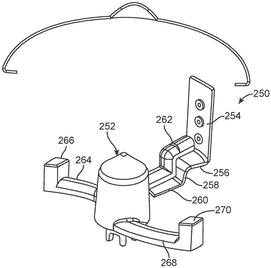
FIG. 2C (PRIOR ART)
