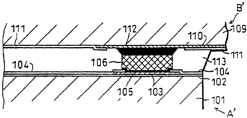
FIG. 13(a) (PRIOR ART)
