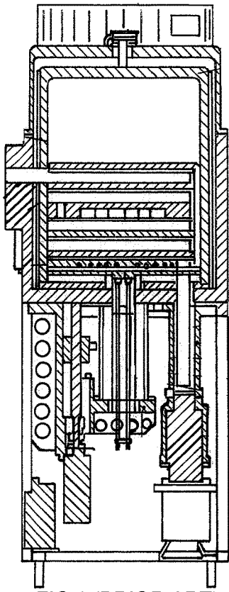
FIG. 1 (PRIOR ART)
