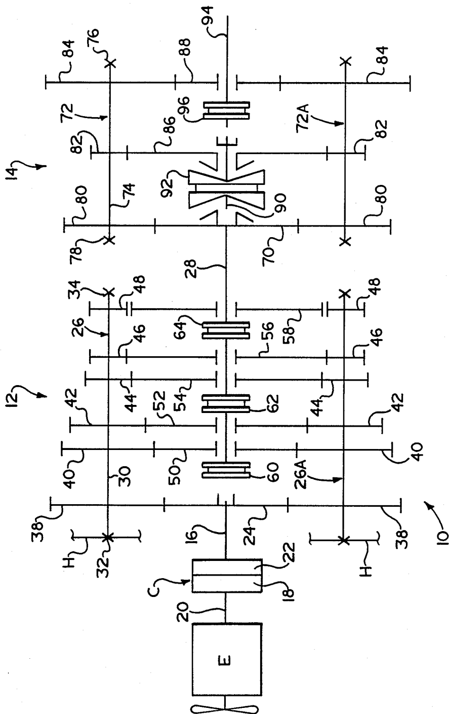
FIG. 1 PRIOR ART
