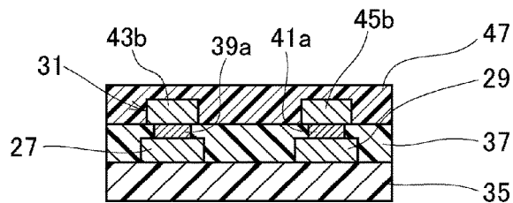
FIG.4D S4 FORM COVER INSULATING LAYER
