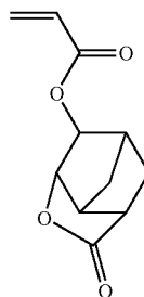
[Chemical Formula 69.]
