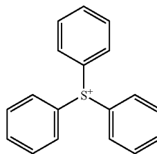
[Chemical Formula 14.]
