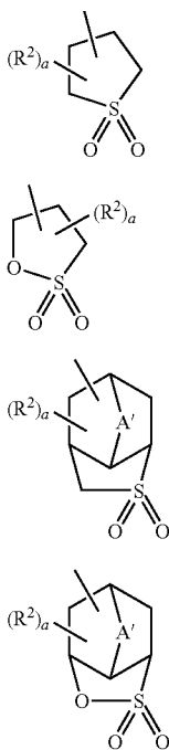
[Chemical Formula 4.]
