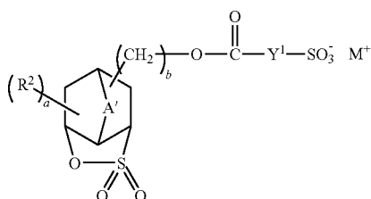
[Chemical Formula 9.]
