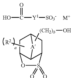
[Chemical Formula 10.]
