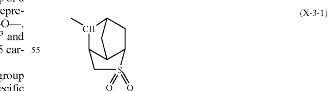
[Chemical Formula 6.]
