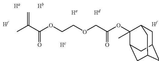
[Chemical Formula 68.]
