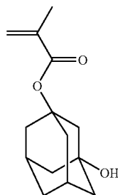
[Chemical Formula 70.]
