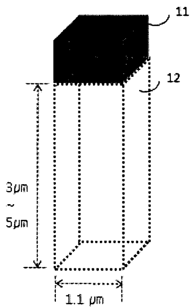
Fig.2 (Prior Art)
