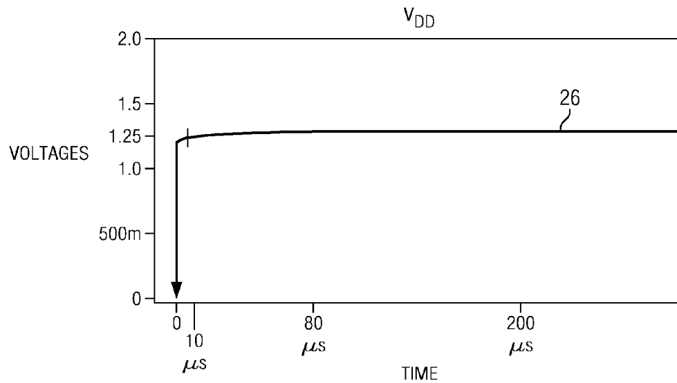
FIG. 3 (PRIOR ART)
