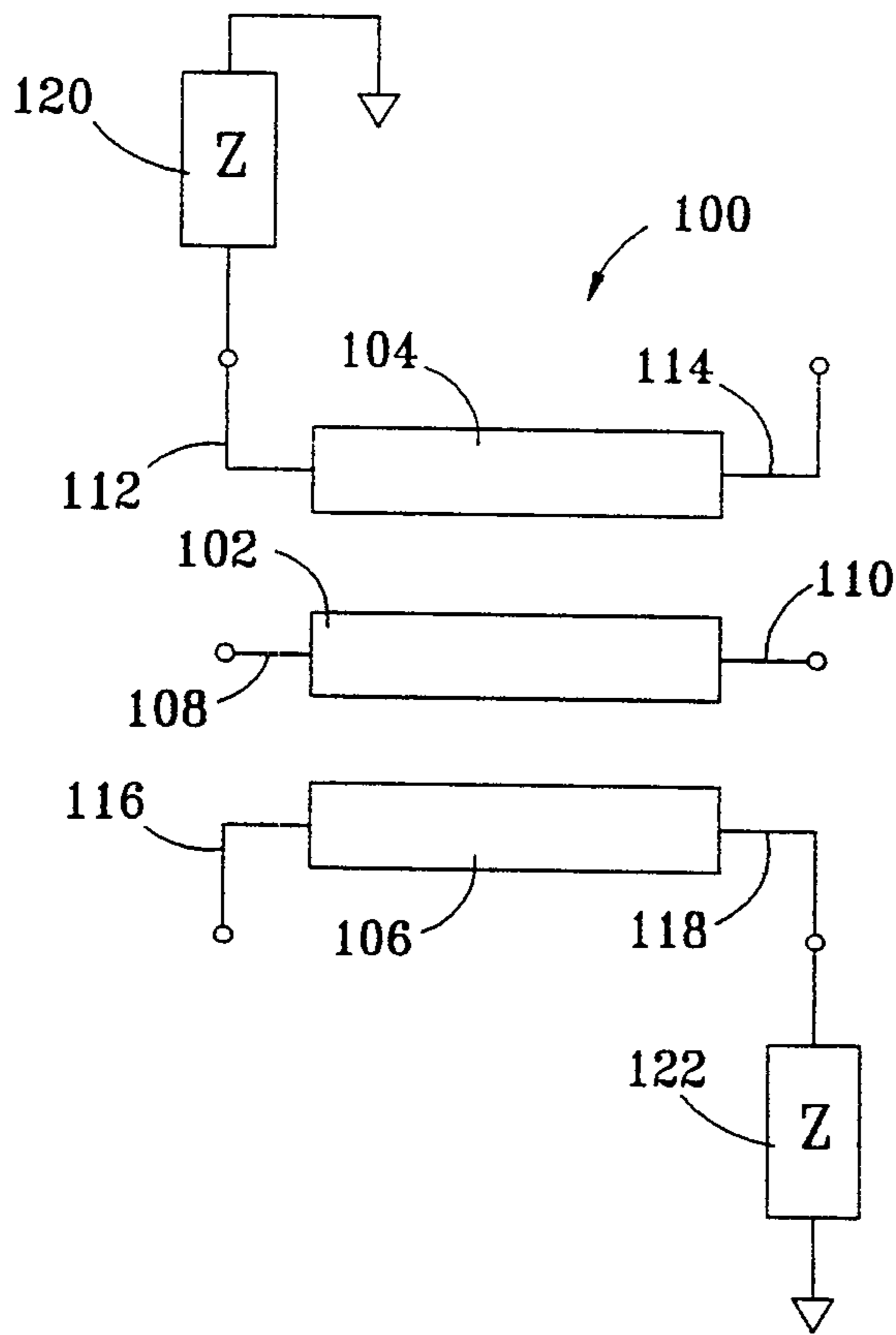
FIG. 4 (PRIOR ART)
