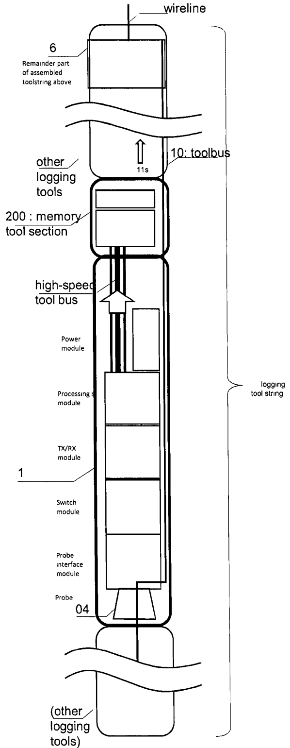
Fig. 10b Generalized logging tool with comm. to surface via signal cable and with one (or more) high data volume producing tools (each) connected to a memory tool.
