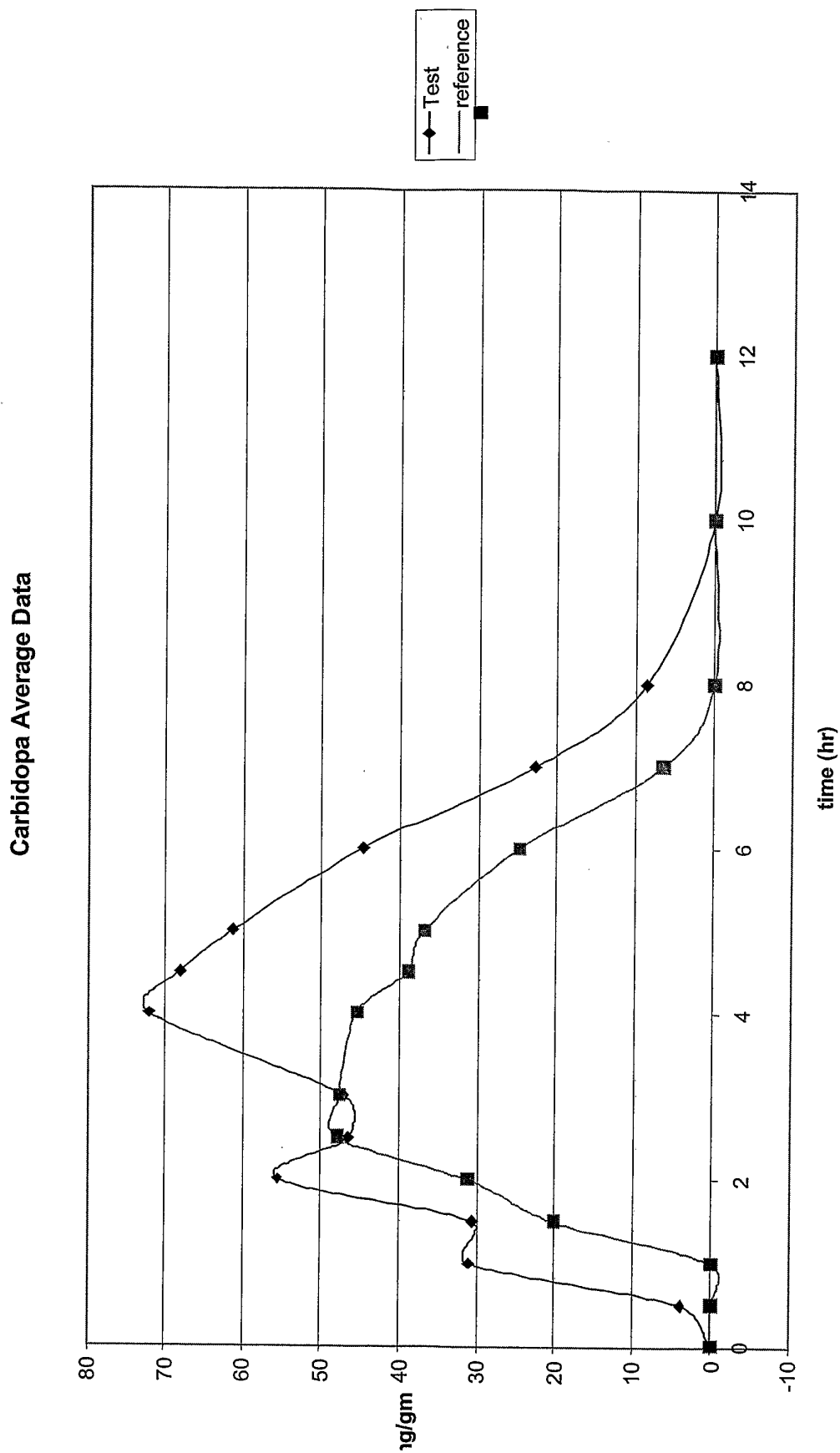
Figure 3 Average Data of Plasma Concentration of Carbidopa versus Time
