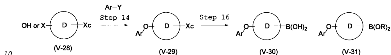
Reaction scheme 10
