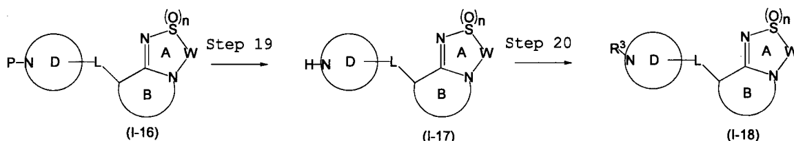
Reaction scheme 6
