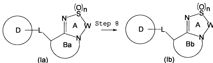
Reaction Scheme 2
