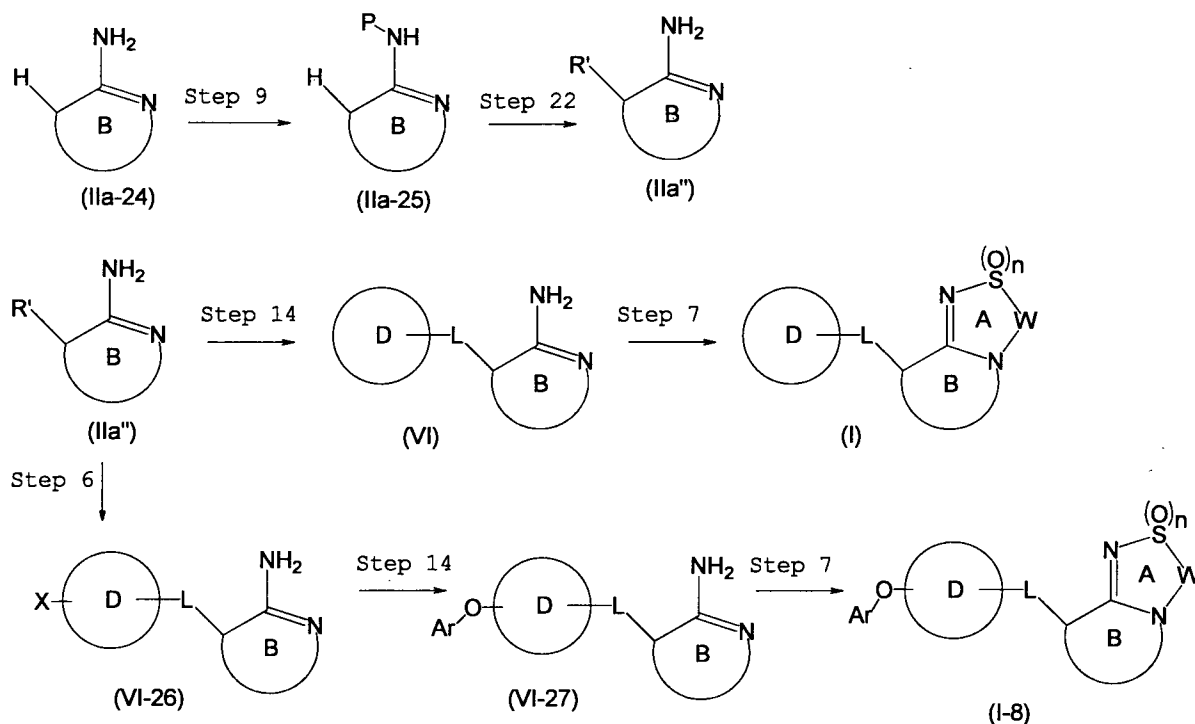
Reaction scheme 9
