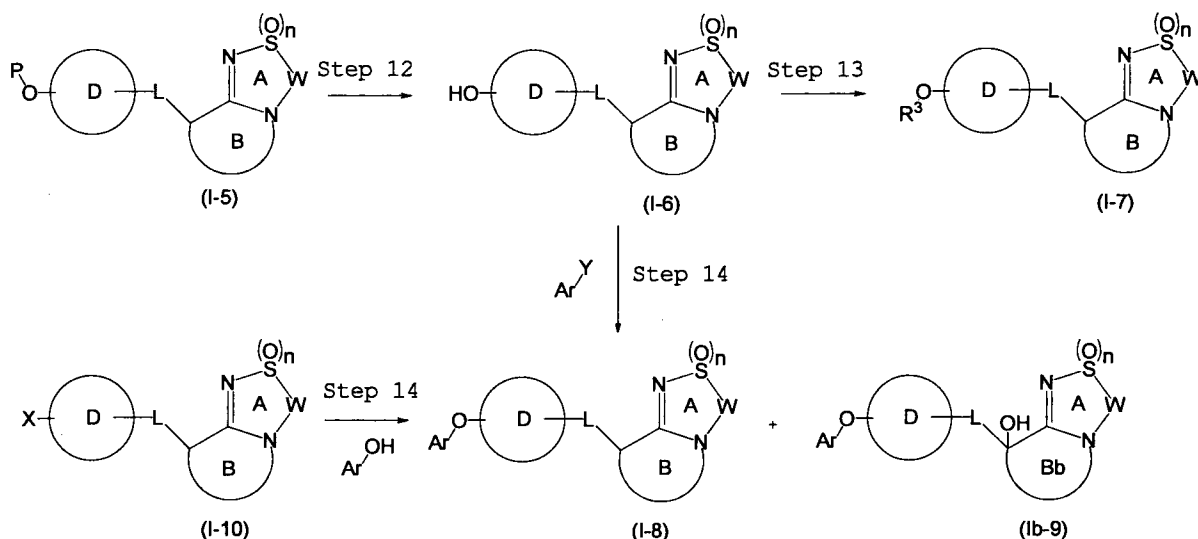
Reaction Scheme 4
