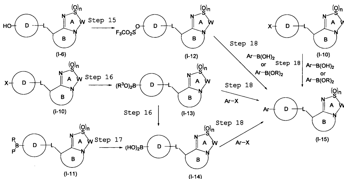
Reaction scheme 5
