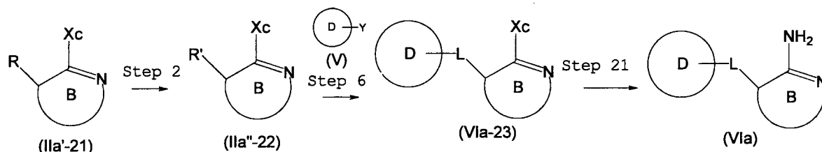
Reaction Scheme 8
