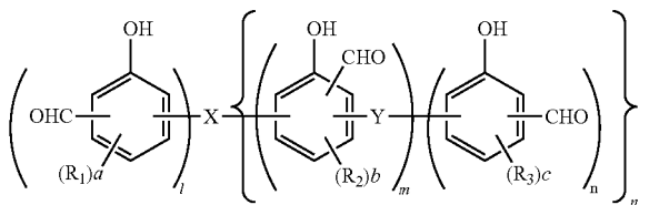
General Formula (2)
