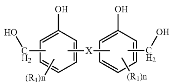
General Formula (6)
