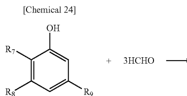
Reaction Formula 1
