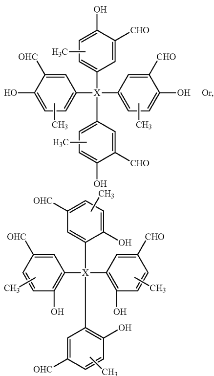
General Formula (19)
