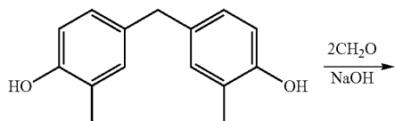
[Chemical 39]
