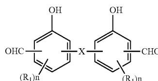
General Formula (4)
