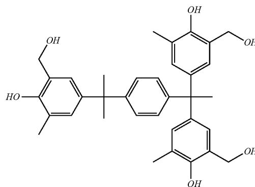
Reaction Formula (7)
