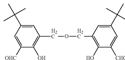
Compound 2
