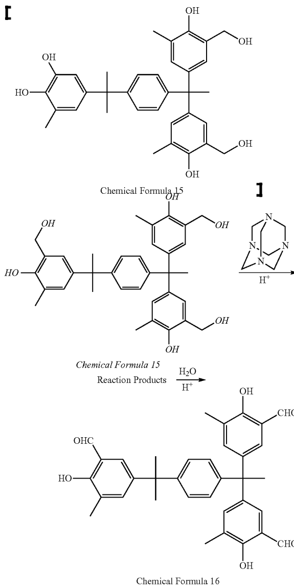
Reaction Formula (3)
