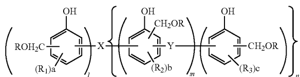
General Formula (1)
