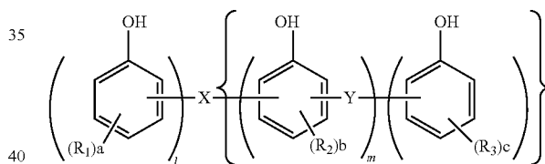
[Chemical 42]
