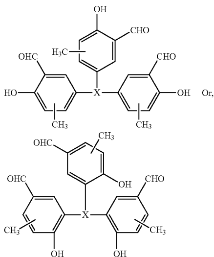
General Formula (17)
