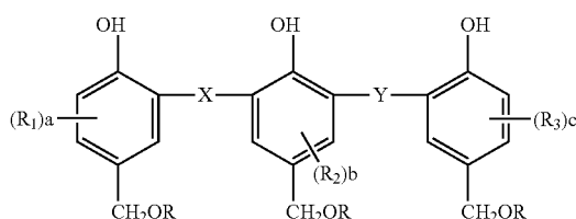
General Formula (22)
