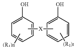
General Formula (5)
