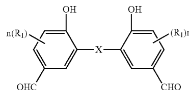
General Formula (14)
