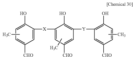
General Formula (19)
