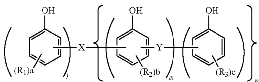
General Formula (10)
