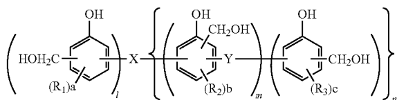
General Formula (11)
