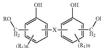
General Formula (3)
