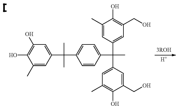
Reaction Formula (7)
