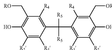
General Formula (16)
