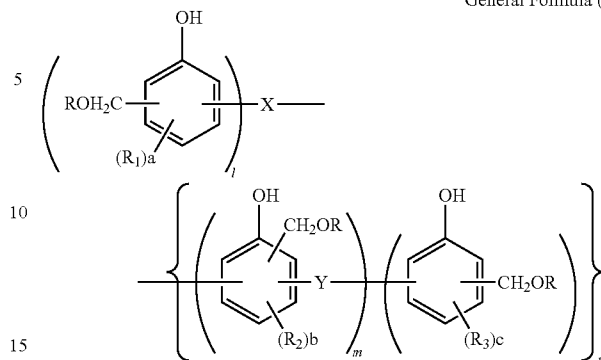
General Formula (1)
