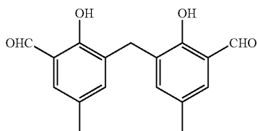
Chemical Formula 18
