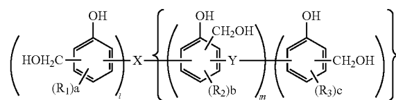
General Formula (11)
