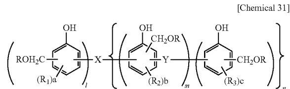
General Formula (8)
