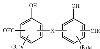
General Formula (4)
