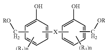
General Formula (3)
