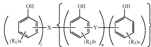
General Formula (10)
