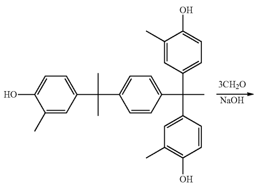
Reaction Formula (6)
