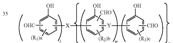
General Formula (2)
