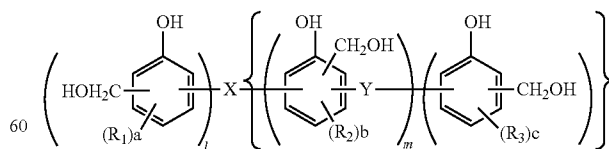
[Chemical 43]
