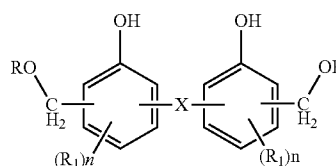
General Formula (3)
