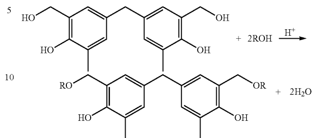
[Chemical 41]
