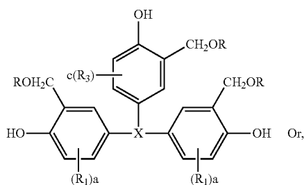
General Formula (20)
