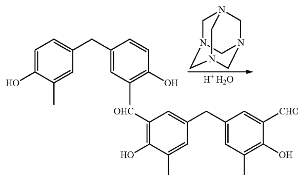
Reaction Formula (8)
