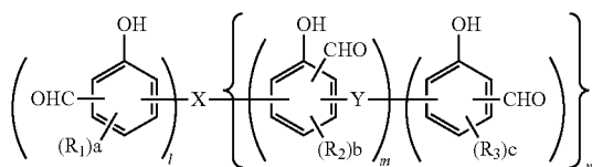
General Formula (9)
