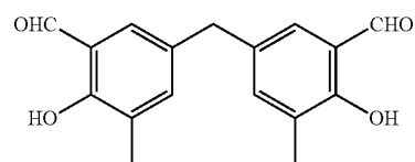
Chemical Formula 17
