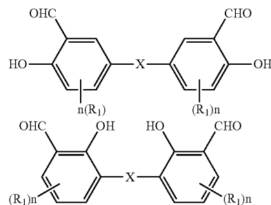
General Formula (13)
