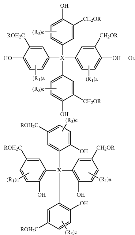
General Formula (21)
