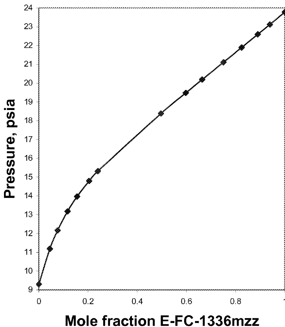
FIGURE 1. E-FC-1336mzz and Methyl Formate at 20 C
