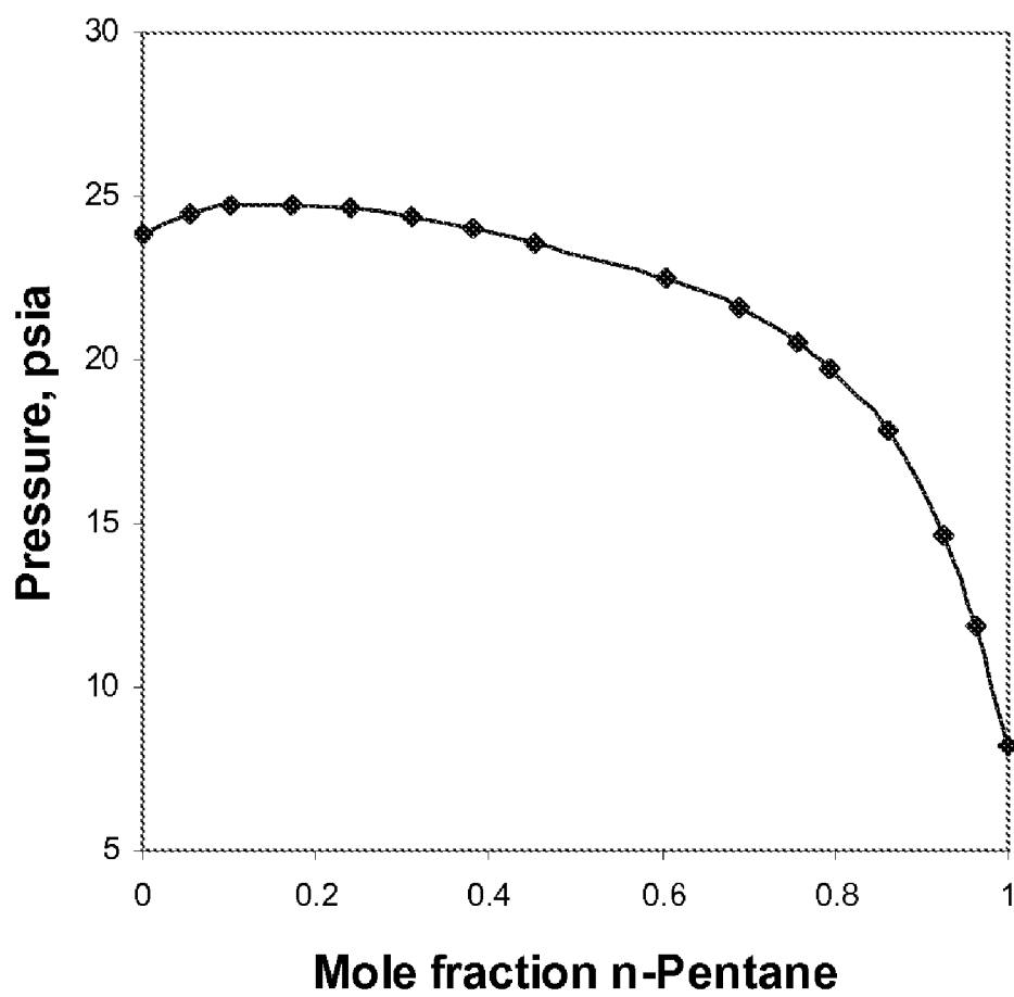
Figure 2. E-FC-1336mzz and n-Pentane at 20 C
