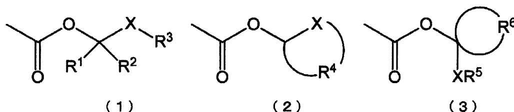
[Chem. 1]
