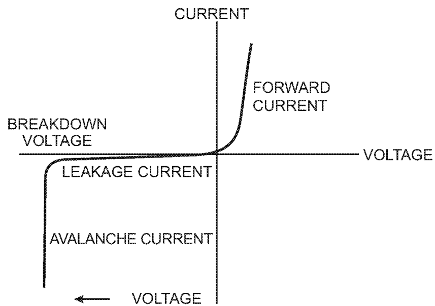
Current-voltage characteristics of a typical P-N junction
