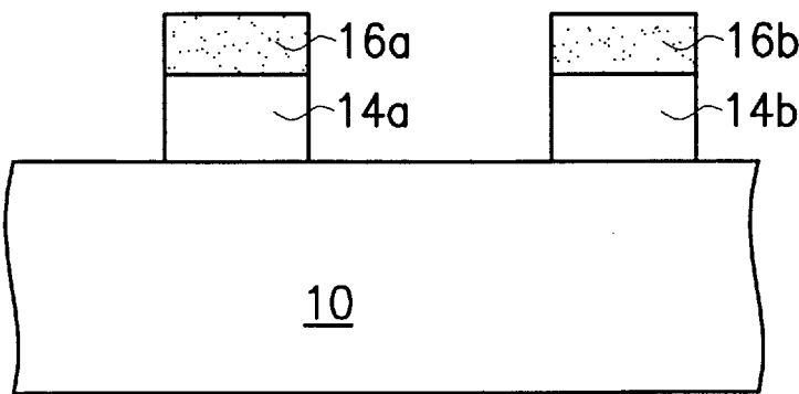
FIG. 1C (PRIOR ART)
