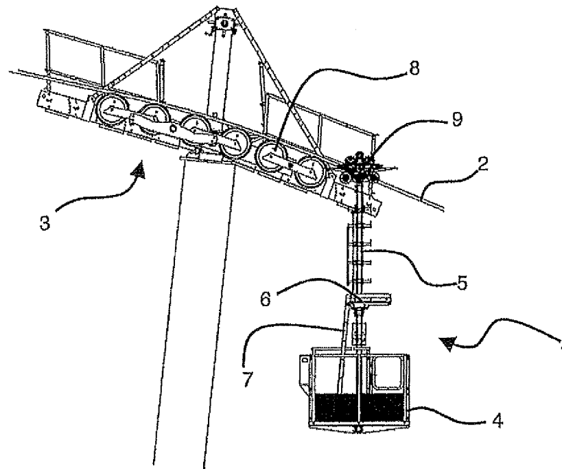
Figure 1 (Prior Art)
