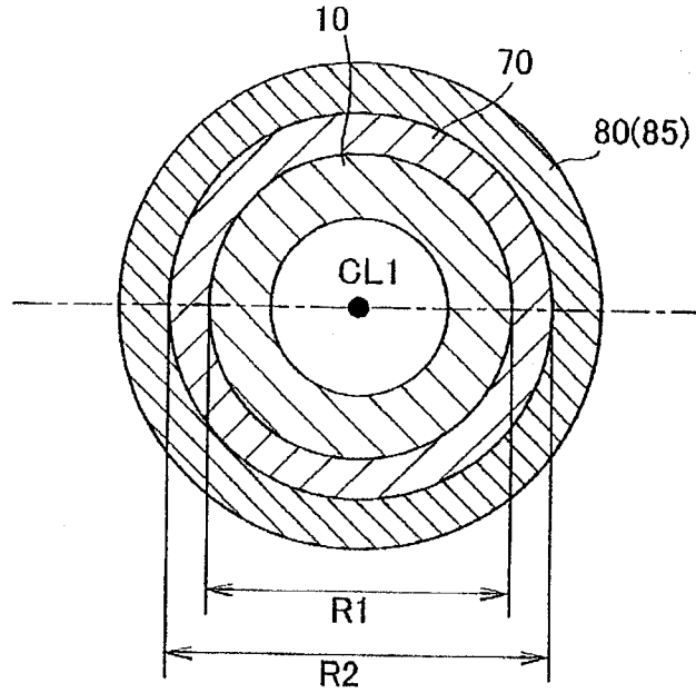
(a) A-A CROSS SECTION
