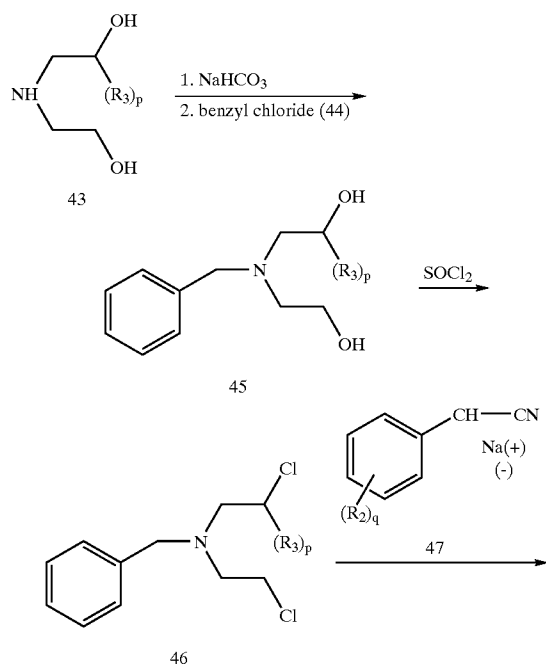
Scheme 10
