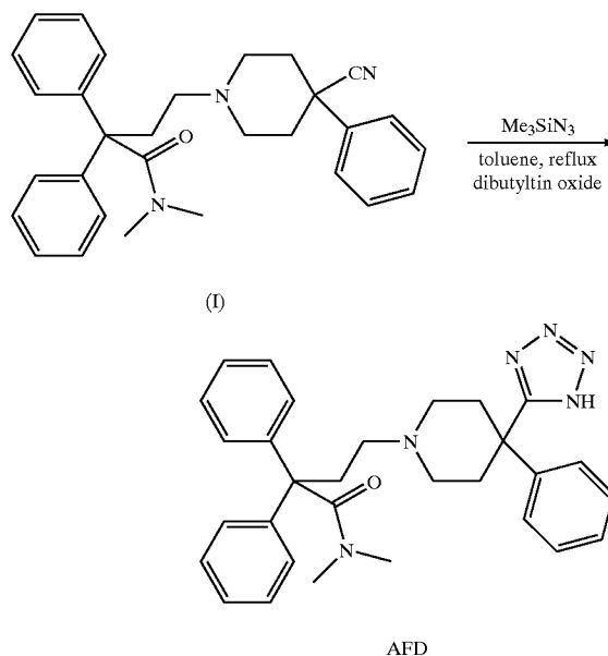
Scheme 20
