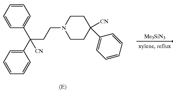
Scheme 14
