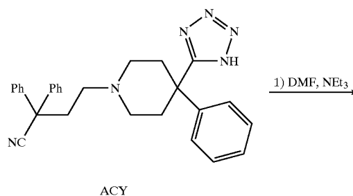
Scheme 16
