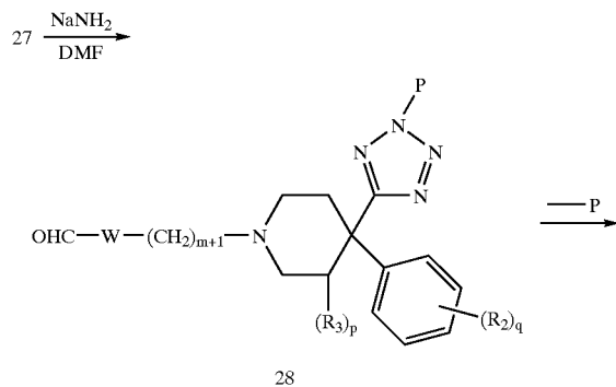
Scheme 6
