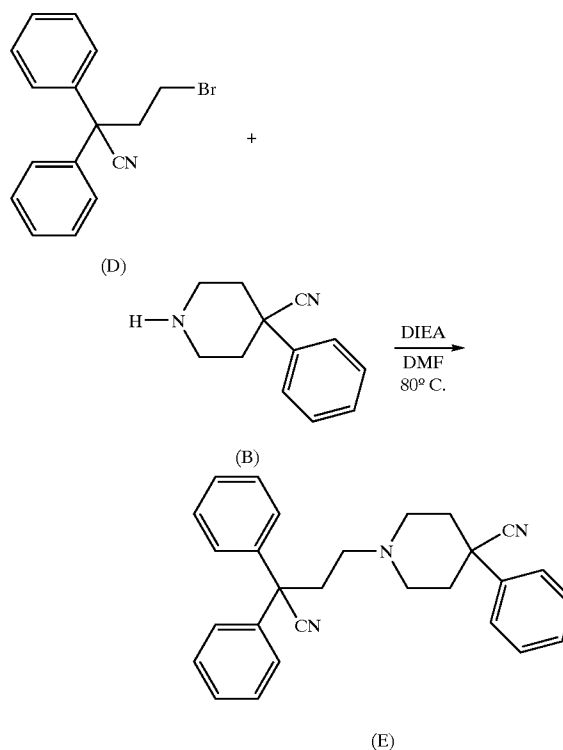
Scheme 13
