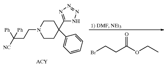
Scheme 15
