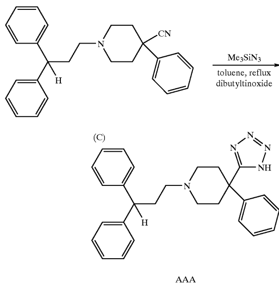
Scheme 12
