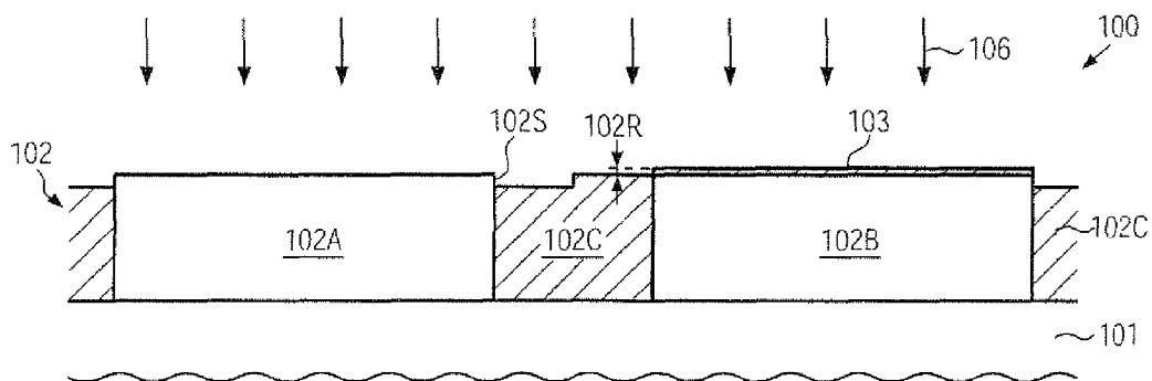
FIG. 1c (prior art)
