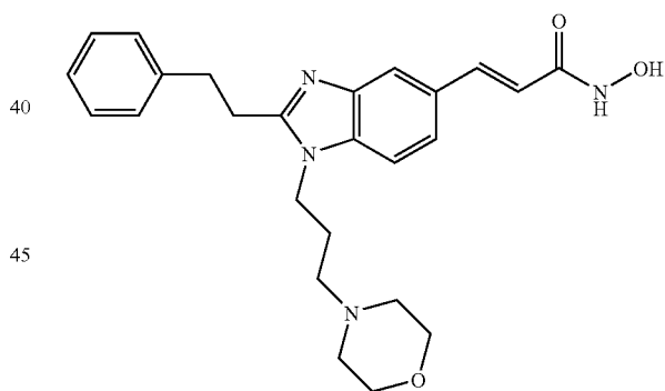
N-Hydroxy-3-[1-(3-morpholin-4-propyl)-2-phenethyl-1H-benzimidazol-5-yl]-acrylamide
