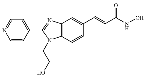
N-Hydroxy-3-[1-(2-hydroxy-ethyl)-2-(4-pyridyl)-1H-benzimidazol-5-yl]-acrylamide
