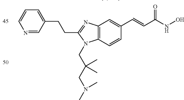
N-Hydroxy-3-[1-(3-Dimethylamino-2,2-dimethyl-propyl)-2-(2-pyridin-3-yl-ethyl)-1H-benzimidazol-5-yl]-acrylamide
