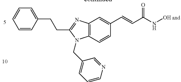
N-Hydroxy-3-[1-(3-pyridylmethyl)-2-(2-phenyl-ethyl)-1H-benzimidazol-5-yl]-acrylamide
