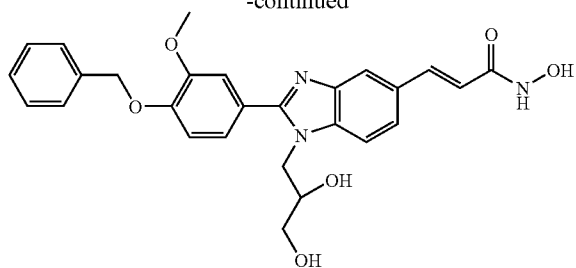
N-Hydroxy-3-[2-(4-benzyloxy-3-methoxy-phenyl)-1-(2,3-hydroxy-propyl)-1H-benzimidazole-5-yl]-acrylamide
