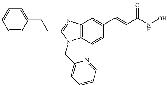
N-Hydroxy-3-(2-phenethyl-1-(pyridin-2-yl)methyl-1H-benzimidazol-5-yl)-acrylamide
