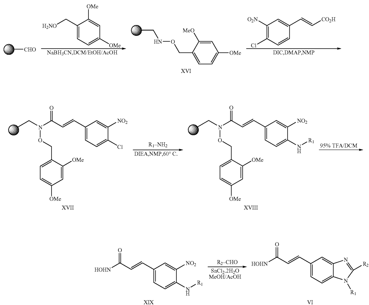
Scheme III
