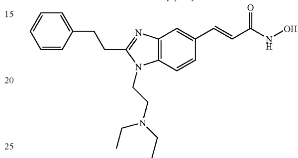
N-Hydroxy-3-[1-(2-diethylamino-ethyl)-2-phenethyl-1H-benzimidazol-5-yl]-acrylamide
