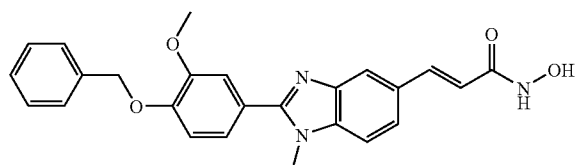
N-Hydroxy-3-[2-(4-benzyloxy-3-methoxy-phenyl)-1-methyl-1H-benzimidazol-5-yl]-acrylamide
