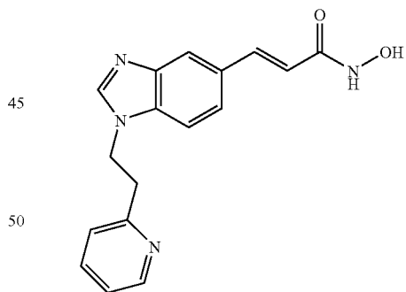
N-Hydroxy-3-[1-(2-pyridin-2-yl-ethyl)-1H-benzimidazol-5-yl]-acrylamide
