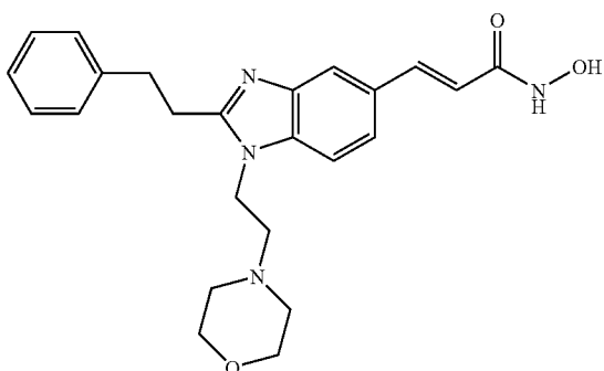
N-Hydroxy-3-[1-(2-morpholin-4-yl-ethyl)-2-phenethyl-1H-benzimidazol-5-yl]-acrylamide
