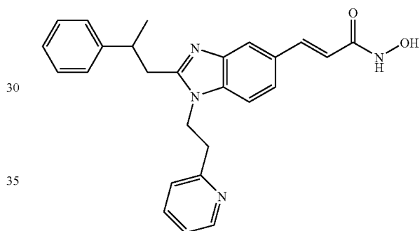
N-Hydroxy-3-[2-(2-phenyl-propyl)-1-(2-pyridin-3-yl-ethyl)-1H-benzimidazol-5-yl]-acrylamide
