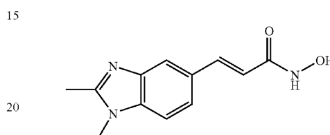
N-Hydroxy-3-(1,2-dimethyl-1H-benzimidazol-5-yl)-acrylamide
