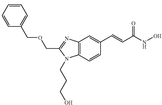
N-Hydroxy-3-[2-Benzyloxymethyl-1-(3-hydroxypropyl)-1H-benzimidazol-5-yl]-acrylamide
