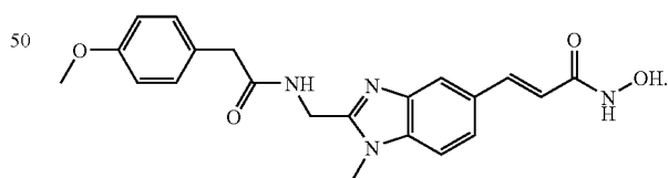
N-Hydroxy-3-(2-{[2-(4-methoxy-phenyl)-acetamino]-methyl}-1-methyl-1H-benzimidazol-5-yl)-acrylamide
