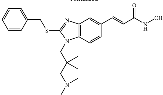
N-Hydroxy-3-[2-benzylsulfanyl-1-(3-dimethylamino-2,2-dimethyl-propyl)-1H-benzimidazol-5-yl]-acrylamide
