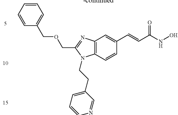
N-Hydroxy-3-[2-Benzyloxymethyl-1-(2-pyridin-3-ethyl)-1H-benzimidazol-5-yl]-acrylamide
