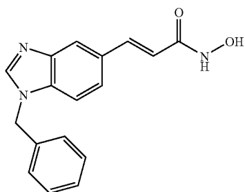
N-Hydroxy-3-(1-benzyl-1H-benzimidazol-5-yl)-acrylamide
