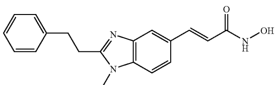
N-Hydroxy-3-(1-methyl-2-phenethyl-1H-benzimidazol-5-yl)-acrylamide
