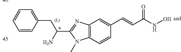
(L)-N-Hydroxy-3-[2-(1-amino-2-phenyl-ethyl)-1-methyl-1H-benzimidazol-5-yl]-acrylamide
