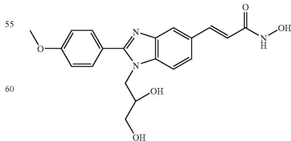
N-Hydroxy-3-[1-(2,3-dihydroxy-propyl)-2-(4-methoxy-phenyl)-1H-benzimidazole-5-yl]-acrylamide
