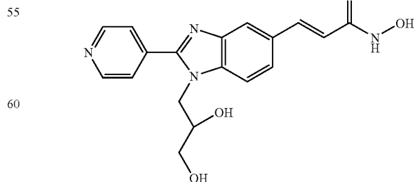
N-Hydroxy-3-[1-(2,3-hydroxy-propyl)-2-(4-pyridyl)-1H-benzimidazol-5-yl]-acrylamide
