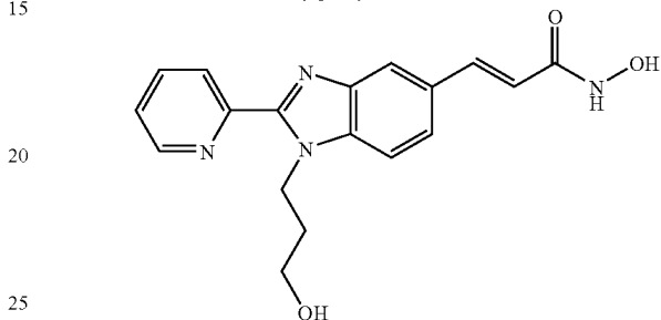
N-Hydroxy-3-[1-(3-hydroxy-propyl)-2-(2-pyridyl)-1H-benzimidazol-5-yl]-acrylamide.
