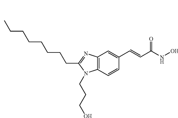
N-Hydroxy-3-[1-(3-hydroxypropyl)-2-octyl-1H-benzimidazol-5-yl]-acrylamide
