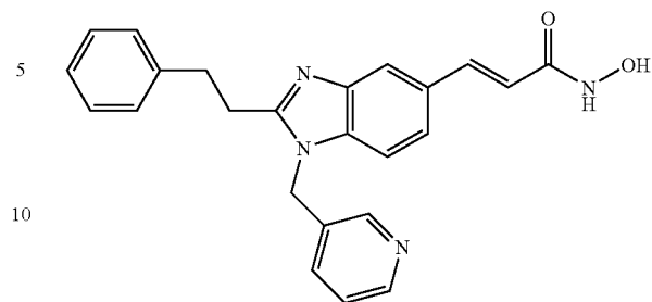
N-Hydroxy-3-[1-(3-pyridylmethyl)-2-(2-phenyl-ethyl)-1H-benzimidazol-5-yl]-acrylamide
