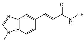
N-Hydroxy-3-(1-methyl-1H-benzimidazol-5-yl)-acrylamide
