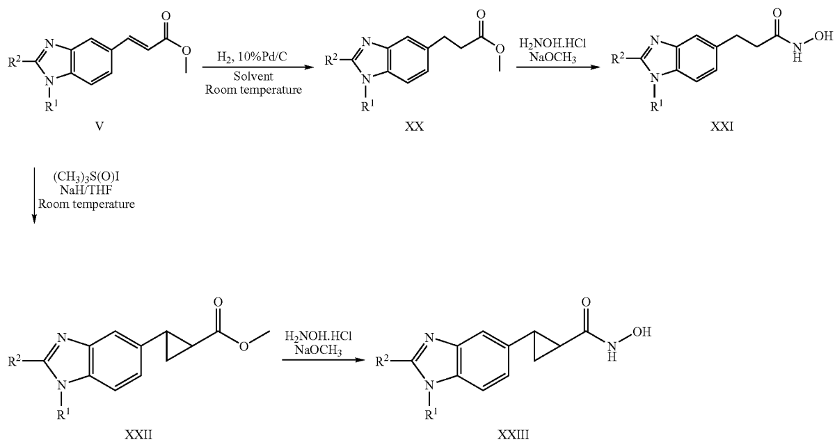
Scheme IV
