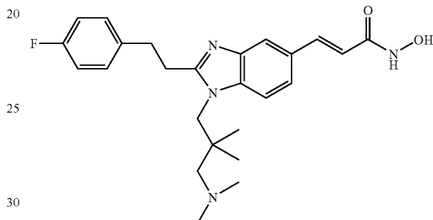
N-Hydroxy-3-(1-(3-Dimethylamino-2,2-dimethyl-propyl)-2-[2-(4-fluoro-phenyl)-ethyl]-1H-benzimidazol-5-yl)-acrylamide
