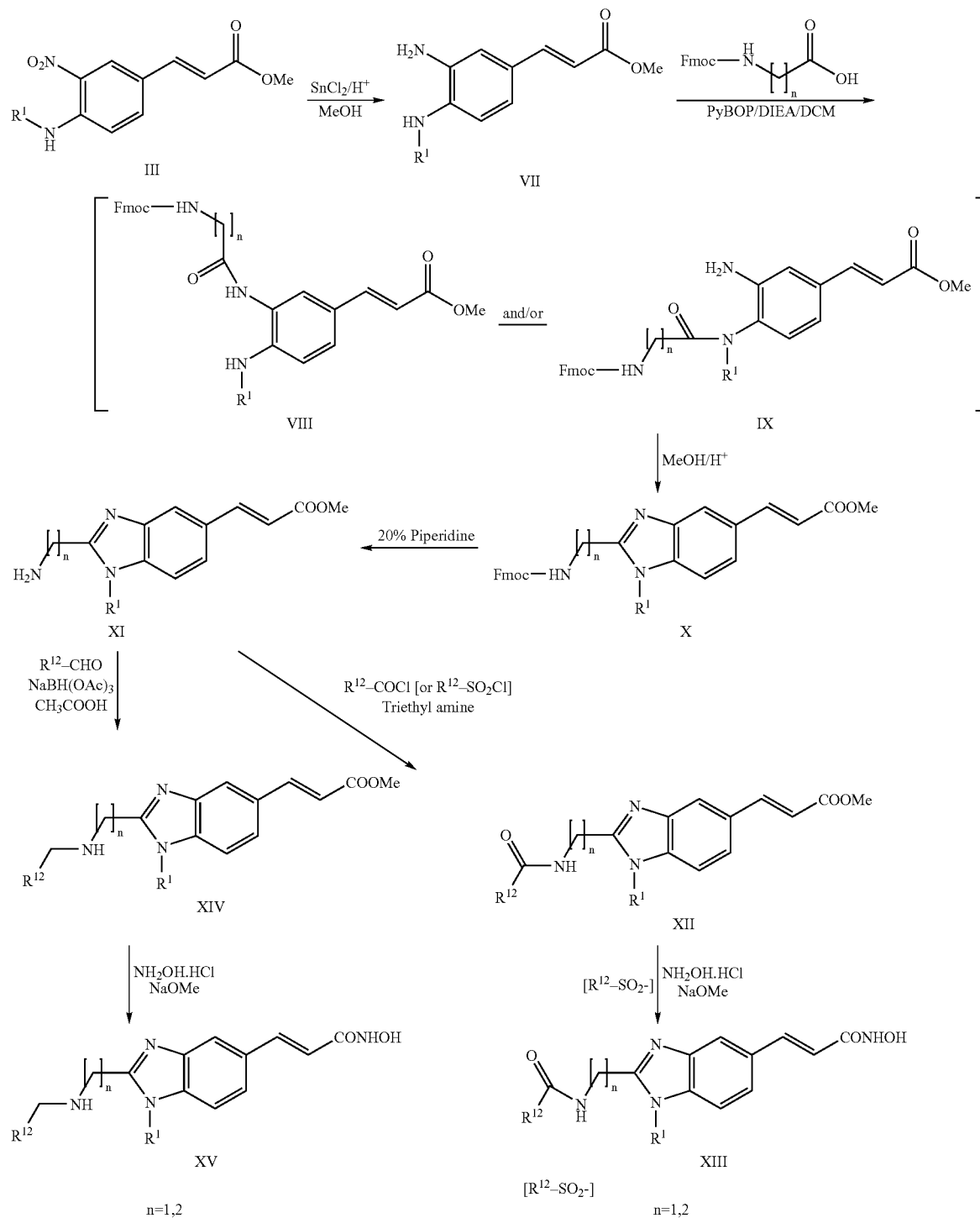
Scheme II
