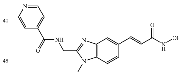
N-[5-(2-Hydroxycarbonyl-vinyl)-1-methyl-1H-benzimidazol-2-ylmethyl]-isonicotinamide
