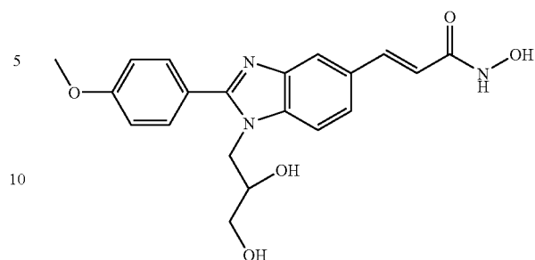
N-Hydroxy-3-[1-(2,3-hydroxy-propyl)-2-(4-methoxy-phenyl)-1H-benzimidazol-5-yl]-acrylamide
