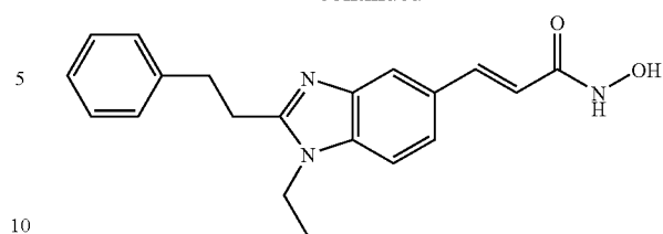
N-Hydroxy-3-(1-Ethyl-2-phenethyl-1H-benzimidazol-5-yl)-acrylamide
