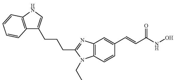
N-Hydroxy-3-(1-ethyl-2-[3-(1H-indol-3-yl)-propyl]-1H-benzimidazol-5-yl)-acrylamide
