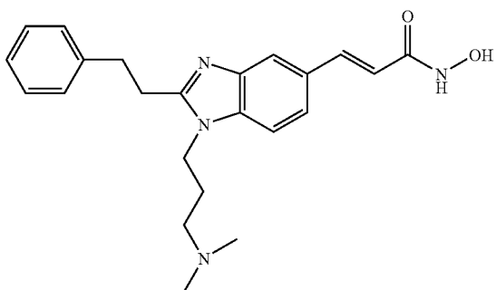
N-Hydroxy-3-[1-(3-dimethylamino-propyl)-2-phenethyl-1H-benzimidazol-5-yl]-acrylamide
