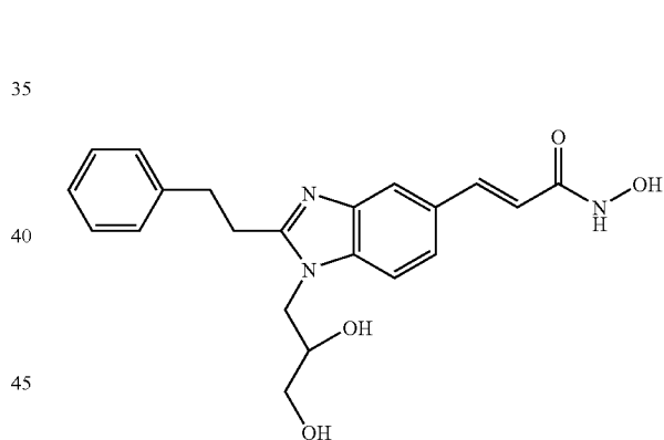
N-Hydroxy-3-[1-(2,3-hydroxy-propyl)-2-(2-phenyl-ethyl)-1H-benzimidazol-5-yl]-acrylamide
