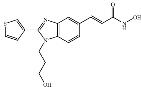
N-Hydroxy-3-[1-(3-hydroxypropyl)-2-thiophen-3-yl-1H-benzimidazol-5-yl]-acrylamide
