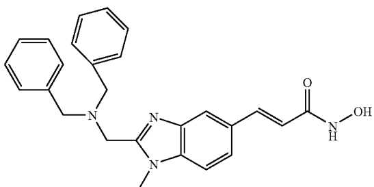
N-Hydroxy-3-{2-[(dibenzylamino)-methyl]-1-methyl-1H-benzimidazol-5-yl}-acrylamide
