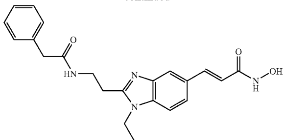
N-Hydroxy-3-[1-ethyl-2-(2-phenylacetyl-amino-ethyl)-1H-benzimidazol-5-yl]-acrylamide
