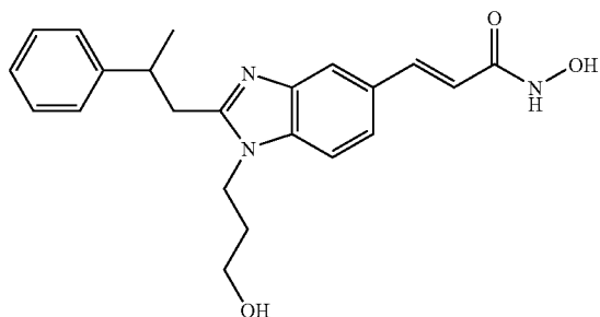
N-Hydroxy-3-[1-(3-hydroxy-propyl)-2-(2-phenyl-propyl)-1H-benzimidazol-5-yl]-acrylamide
