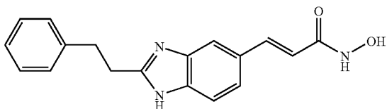
N-Hydroxy-3-(2-phenethyl-1H-benzimidazol-5-yl)-acrylamide
