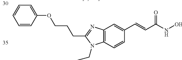
N-Hydroxy-3-[1-ethyl-2-(3-phenoxy-propyl)-1H-benzimidazol-5-yl]-acrylamide
