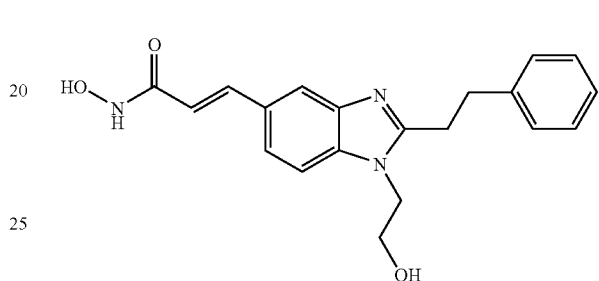
N-Hydroxy-3-[1-(2-hydroxyethyl)-2-phenethyl-1H-benzimidazol-5-yl]-acrylamide
