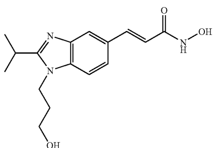
N-Hydroxy-3-[1-(3-hydroxy-propyl)-2-isopropyl-1H-benzimidazol-5-yl]-acrylamide
