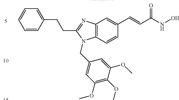
N-Hydroxy-3-[1-(3,4,5-trimethoxybenzyl)-2-(2-phenyl-ethyl)-1H-benzimidazol-5-yl]-acrylamide
