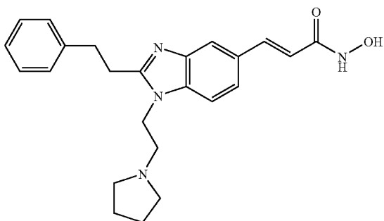
N-Hydroxy-3-[2-phenylethyl-1-(2-pyrrolidin-1-yl-ethyl)-1H-benzimidazol-5-yl]-acrylamide
