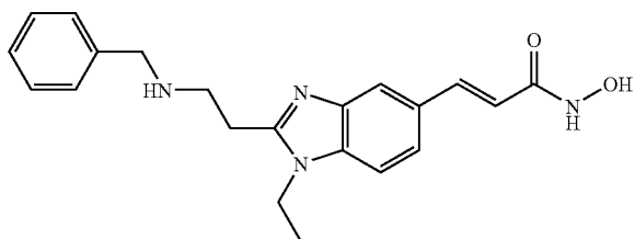
N-Hydroxy-3-[2-(2-benzylamino-ethyl)-1-ethyl-1H-benzimidazol-5-yl]-acrylamide
