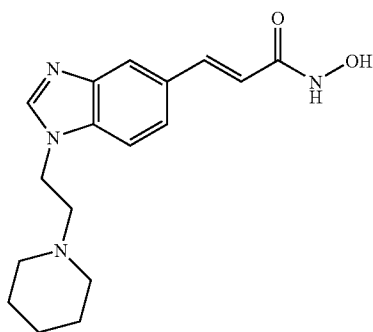
N-Hydroxy-3-[1-(2-piperidin-1-yl-ethyl)-1H-benzimidazol-5-yl]-acrylamide
