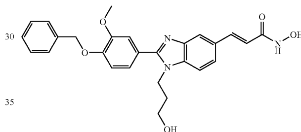
N-Hydroxy-3-[2-(4-benzyloxy-3-methoxy-phenyl)-1-(3-hydroxy-propyl)-1H-benzimidazole-5-yl]-acrylamide
