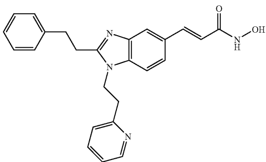
N-Hydroxy-3-[2-phenethyl-1-(2-pyridin-2-yl-ethyl)-1H-benzimidazol-5-yl]-acrylamide
