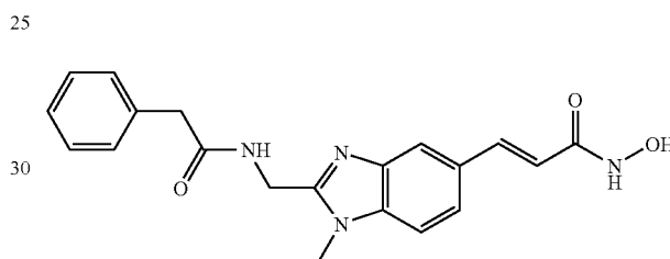
N-Hydroxy-3-[1-methyl-2-(phenylacetylamino-methyl)-1H-benzimidazol-5-yl]-acrylamide
