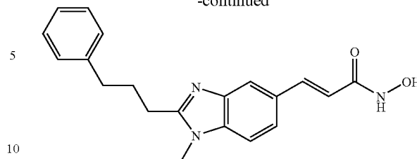
N-Hydroxy-3-[1-methyl-2-(3-phenyl-propyl)-1H-benzimidazol-5-yl]-acrylamide
