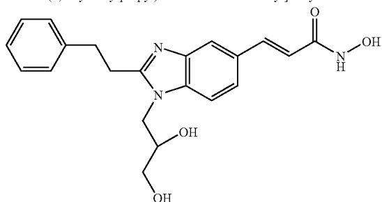
N-Hydroxy-3-[1-(2,3-hydroxy-propyl)-2-(2-phenyl-ethyl)-1H-benzimidazole-5-yl]-acrylamide
