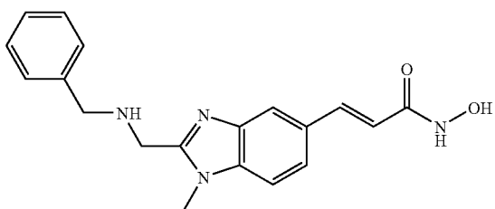
N-Hydroxy-3-[2-(benzylamino-methyl)-1-methyl-1H-benzimidazol-5-yl]-acrylamide
