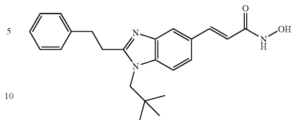
N-Hydroxy-3-[1-(2,2-dimethyl-propyl)-2-phenethyl-1H-benzimidazol-5-yl]-acrylamide
