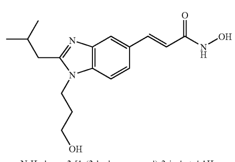
N-Hydroxy-3-[1-(3-hydroxypropyl)-2-isobutyl-1H-benzimidazol-5-yl]-acrylamide
