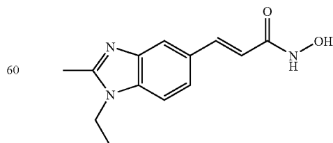
N-Hydroxy-3-(1-Ethyl-2-methyl-1H-benzimidazol-5-yl)-acrylamide
