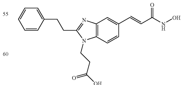
3-[5-(2-Hydroxycarbonyl-vinyl)-2-phenethyl-1H-benzimidazol-1-yl]-propionic acid
