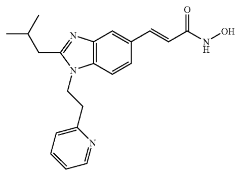
N-Hydroxy-3-[2-isobutyl-1-(2-pyridin-2-yl-ethyl)-1H-benzimidazol-5-yl]-acrylamide
