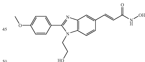
N-Hydroxy-3-[1-(2-hydroxy-ethyl)-2-(4-methoxy-phenyl)-1H-benzimidazole-5-yl]-acrylamide
