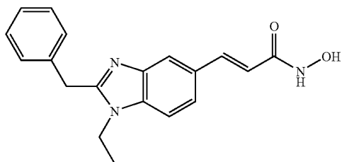
N-Hydroxy-3-(2-benzyl-1-ethyl-1H-benzimidazol-5-yl)-acrylamide
