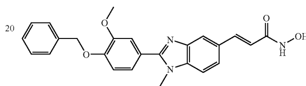
N-Hydroxy-3-[2-(4-benzyloxy-3-methoxy-phenyl)-1-methyl-1H-benzimidazole-5-yl]-acrylamide
