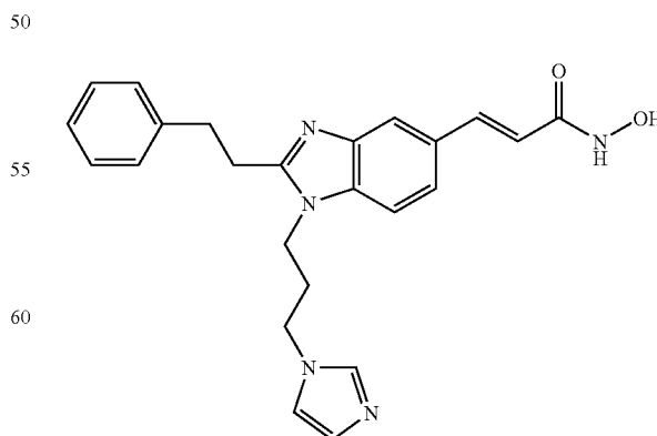
N-Hydroxy-3-[1-(3-imidazol-1-yl-propyl)-2-phenethyl-1H-benzimidazol-5-yl]-acrylamide
