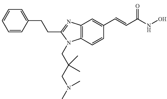
N-Hydroxy-3-[1-(3-Dimethylamino-2,2-dimethylpropyl)-2-phenethyl-1H-benzimidazol-5-yl]-acrylamide
