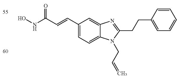
N-Hydroxy-3-(1-allyl-2-phenethyl-1H-benzimidazol-5-yl)-acrylamide
