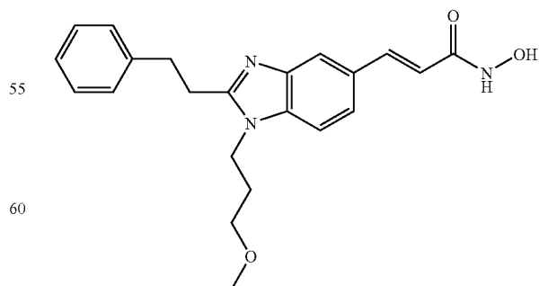
N-Hydroxy-3-[1-(3-methoxy-propyl)-2-phenethyl-1H-benzimidazol-5-yl]-acrylamide
