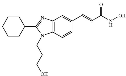
N-Hydroxy-3-[2-cyclohexyl-1-(3-hydroxy-propyl)-1H-benzimidazol-5-yl]-acrylamide
