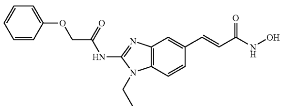
N-Hydroxy-3-[1-ethyl-2-[2-(2-phenoxy-acetyl-amino)-ethyl]-1H-benzimidazol-5-yl]-acrylamide
