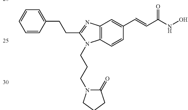
N-Hydroxy-3-[1-[3-(2-oxo-pyrrolidin-1-yl)-propyl]-2-phenethyl-1H-benzimidazol-5-yl]-acrylamide
