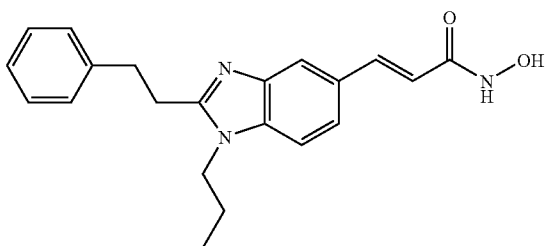
N-Hydroxy-3-(2-phenethyl-1-propyl-1H-benzimidazol-5-yl)-acrylamide
