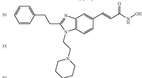
N-Hydroxy-3-[2-phenethyl-1-(piperidin-1-yl-ethyl)-1H-benzimidazol-5-yl]-acrylamide
