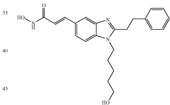
N-Hydroxy-3-[1-(5-hydroxy-pentyl)-2-phenethyl-1H-benzimidazol-5-yl]-acrylamide
