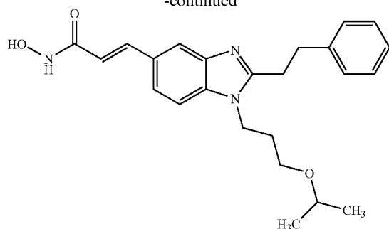
N-Hydroxy-3-(1-(3-isopropoxy-propyl)-2-phenethyl-1H-benzimidazol-5-yl)-acrylamide
