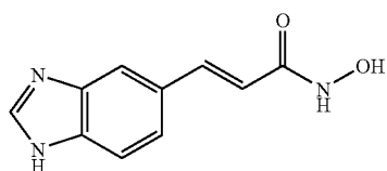
N-Hydroxy-3-(1H-benzimidazol-5-yl)-acrylamide
