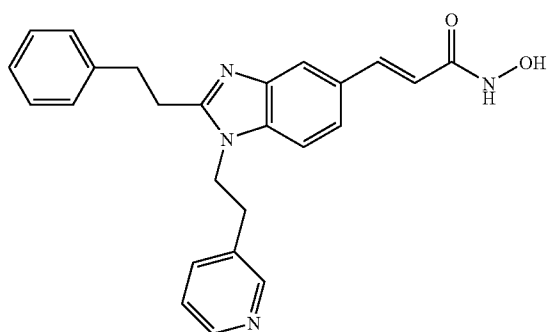
N-Hydroxy-3-(2-phenethyl-1-(2-pyridin-3-yl-ethyl)-1H-benzimidazol-5-yl)-acrylamide
