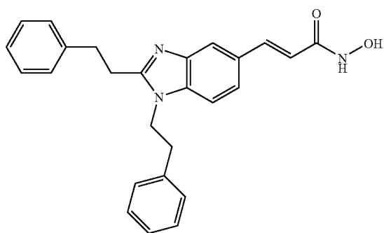
N-Hydroxy-3-(1,2-Diphenethyl-1H-benzimidazol-5-yl)-acrylamide
