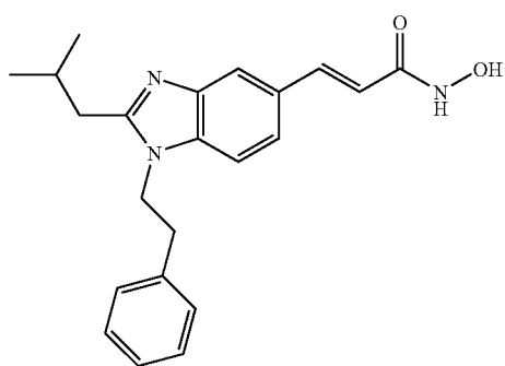
N-Hydroxy-3-(2-isobutyl-1-phenethyl-1H-benzimidazol-5-yl)-acrylamide
