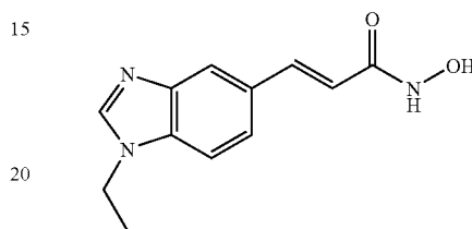
N-Hydroxy-3-(1-Ethyl-1H-benzimidazol-5-yl)-acrylamide
