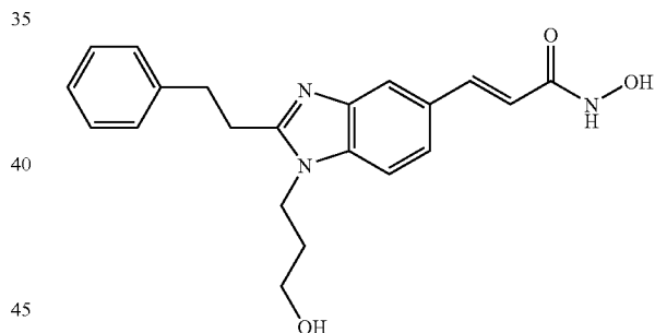
N-Hydroxy-3-[1-(3-hydroxy-propyl)-2-phenethyl-1H-benzimidazol-5-yl]-acrylamide
