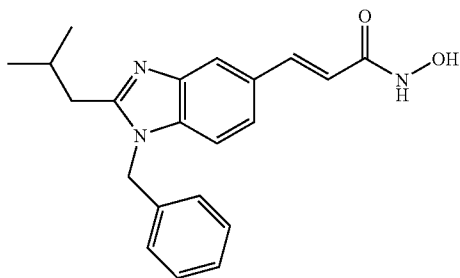
N-Hydroxy-3-(1-Benzyl-2-isobutyl-1H-benzimidazol-5-yl)-acrylamide
