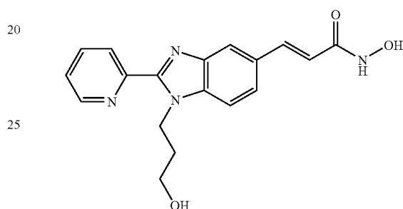
N-Hydroxy-3-[1-(3-hydroxy-propyl)-2-(2-pyridyl)-1H-benzimidazol-5-yl]-acrylamide
