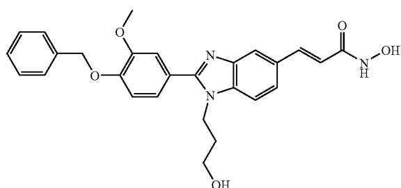
N-Hydroxy-3-[2-(4-benzyloxy-3-methoxy-phenyl)-1-(3-hydroxy-propyl)-1H-benzimidazol-5-yl]-acrylamide
