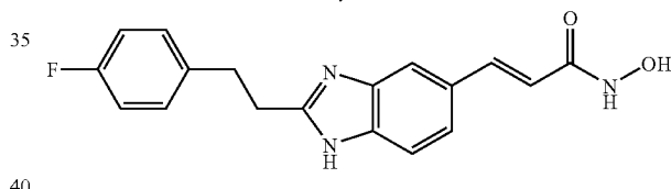
N-Hydroxy-3-[2-(4-fluoro-phenyl)-ethyl]-1H-benzimidazol-5-yl]-acrylamide
