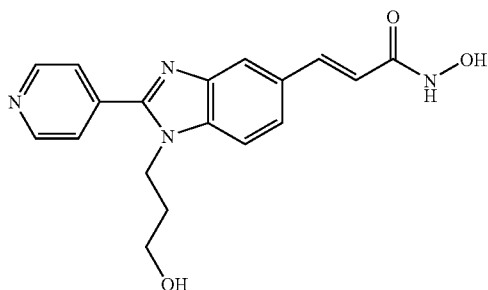
N-Hydroxy-3-[1-(3-hydroxy-propyl)-2-(4-pyridyl)-1H-benzimidazol-5-yl]-acrylamide
