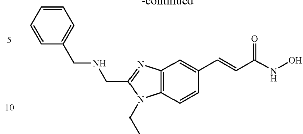
N-Hydroxy-3-[2-(benzylamino-methyl)-ethyl-1H-benzimidazol-5-yl]-acrylamide
