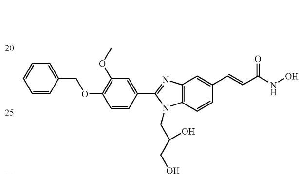
N-Hydroxy-3-[2-(4-benzyloxy-3-methoxy-phenyl)-1-(2,3-hydroxy-propyl)-1H-benzimidazol-5-yl]-acrylamide
