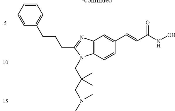
N-Hydroxy-3-[1-(3-Dimethylamino-2,2-dimethyl-propyl)-2-(3-phenyl-propyl)-1H-benzimidazol-5-yl]-acrylamide
