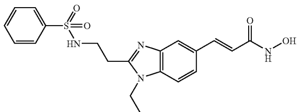
N-Hydroxy-3-[2-(2-benzenesulfonylamino-ethyl)-1-ethyl-1H-benzimidazol-5-yl]-acrylamide
