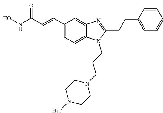
N-Hydroxy-3-(1-[3-(4-methyl-piperzin-1-yl)-2-phenethyl-1H-benzimidazol-5-yl]-acrylamide
