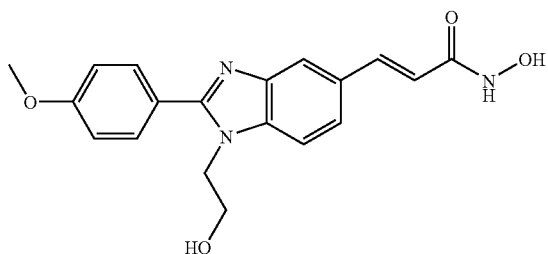
N-Hydroxy-3-[1-(2-hydroxy-ethyl)-2-(4-methoxy-phenyl)-1H-benzimidazol-5-yl]-acrylamide
