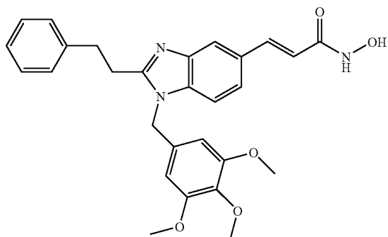
N-Hydroxy-3-[1-(3,4,5-trimethoxybenzyl)-2-(2-phenyl-ethyl)-1H-benzimidazol-5-yl]-acrylamide
