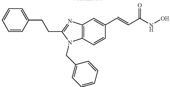
N-Hydroxy-3-(1-Benzyl-2-phenethyl-1H-benzimidazol-5-yl)-acrylamide
