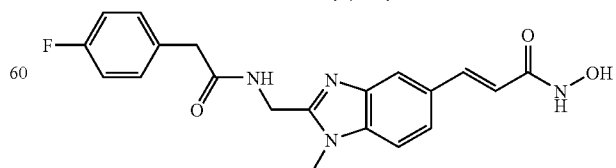
N-Hydroxy-3-(2-[[2-(4-fluoro-phenyl)-acetyl-amino]-methyl]-1-methyl-1H-benzimidazol-5-yl)-acrylamide
