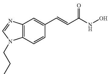
N-Hydroxy-3-(1-propyl-1H-benzimidazol-5-yl)-acrylamide
