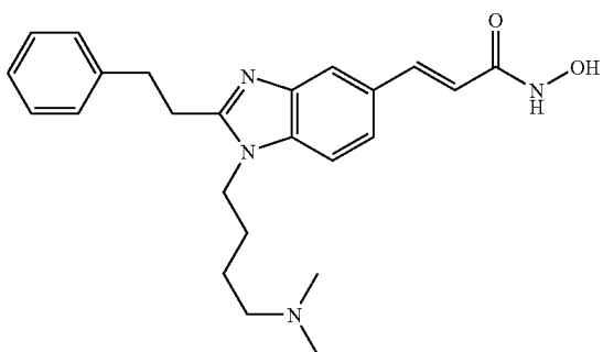
N-Hydroxy-3-[1-(4-dimethylamino-butyl)-2-phenethyl-1H-benzimidazol-5-yl]-acrylamide
