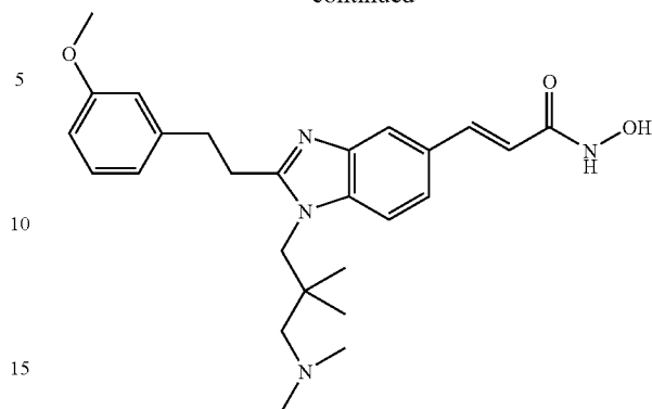
N-Hydroxy-3-(1-(3-dimethylamino-2,2-dimethyl-propyl)-2-[2-(3-methoxy-phenyl)-ethyl]-1H-benzimidazol-5-yl)-acrylamide
