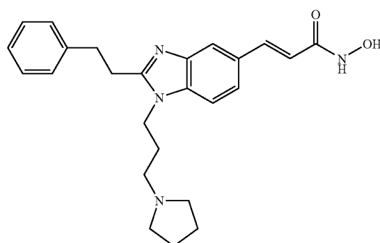
N-Hydroxy-3-[2-phenethyl-1-(3-pyrrolidin-1-yl-propyl)-1H-benzimidazol-5-yl]-acrylamide
