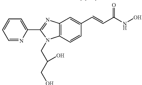
N-Hydroxy-3-[1-(2,3-hydroxy-propyl)-2-(2-pyridyl)-1H-benzimidazol-5-yl]-acrylamide
