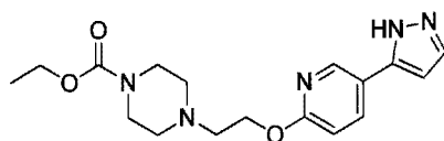
Compound B
