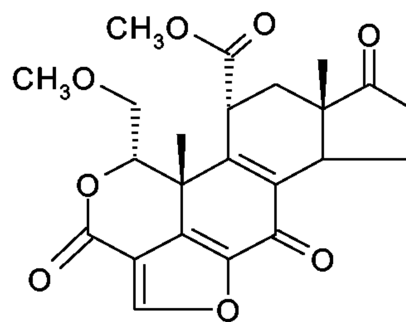
Wortmannin
