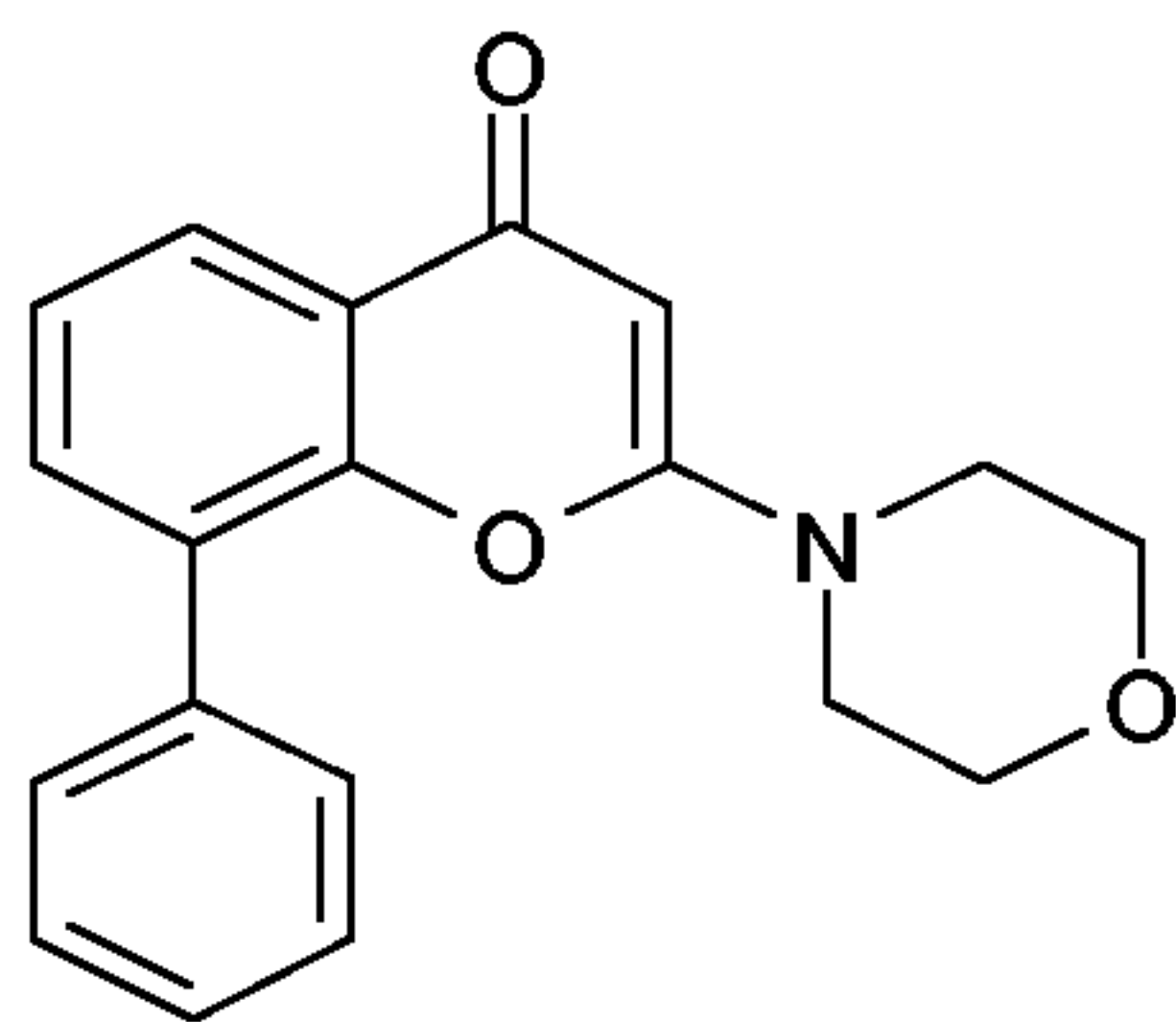
LY 294002
