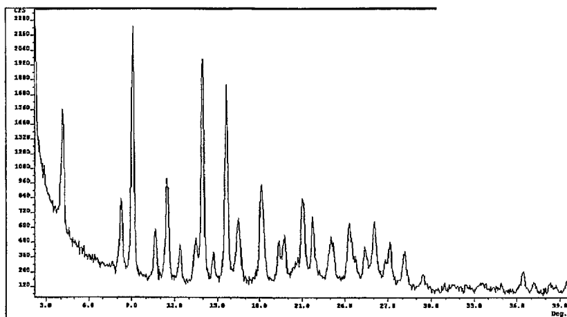
an XRD diffractogram of Tigecycline Form I
