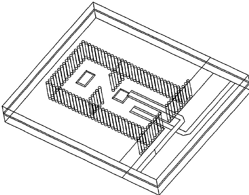
FIG. 4 (PRIOR ART)
