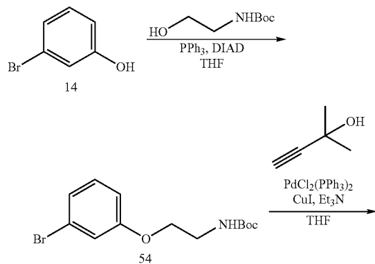
SCHEME 13
