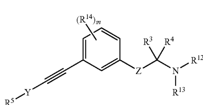
Formula (A)
