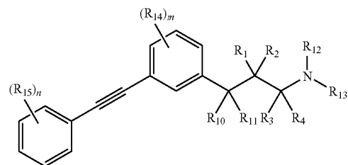
Formula (IIb)
