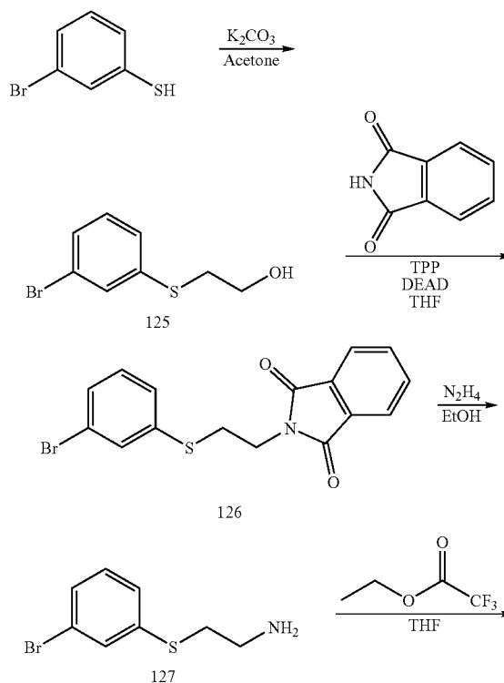
SCHEME 30
