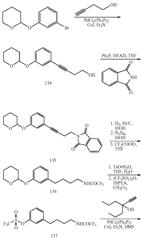
SCHEME 33
