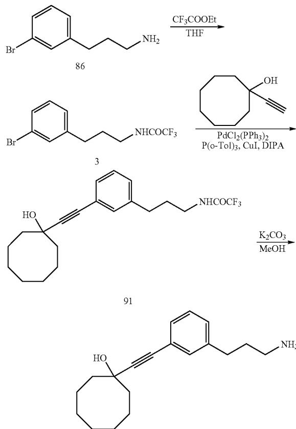
SCHEME 23
