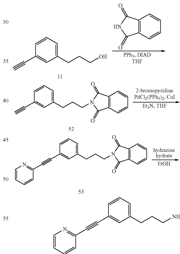
SCHEME 12
