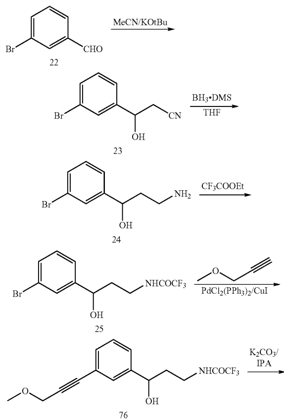
SCHEME 18
