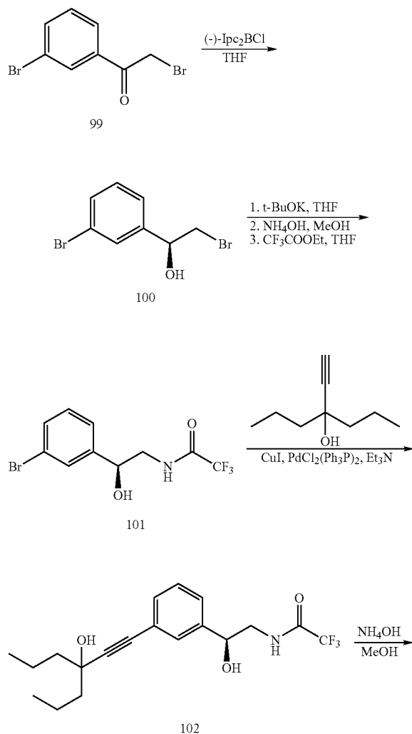
SCHEME 25
