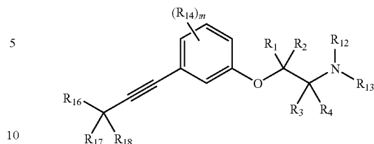
Formula (IIIa)
