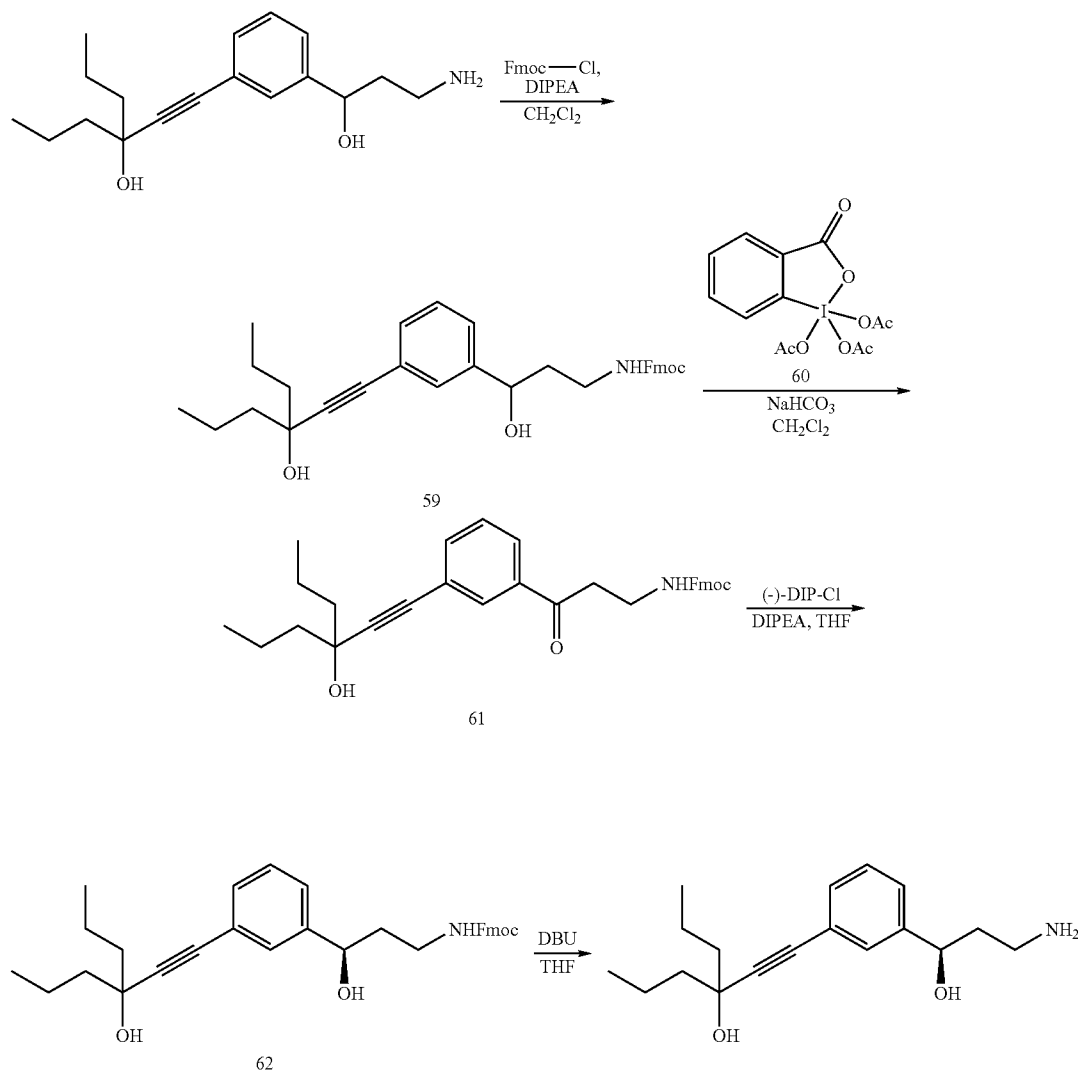
Scheme 15
