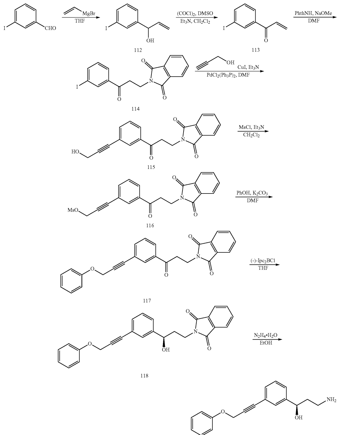
SCHEME 28
