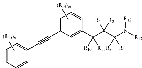
Formula (IIa)
