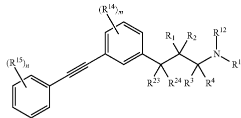
Formula (C)
