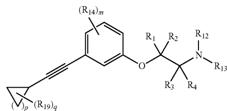
Formula (H)
