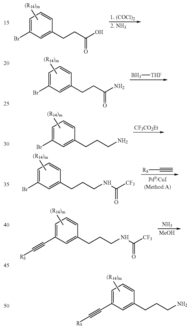
Scheme I
