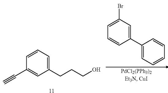
SCHEME 9
