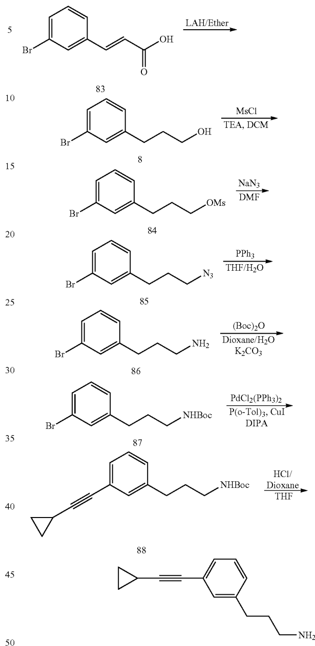
SCHEME 21
