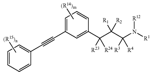
Formula (B)
