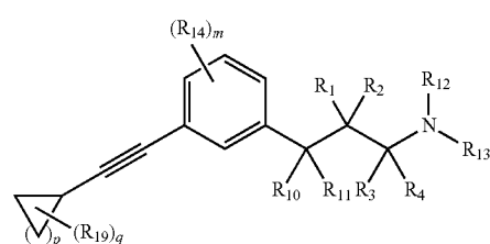
Formula (F)
