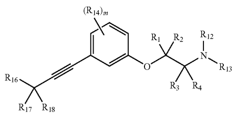
Formula (IIIa)
