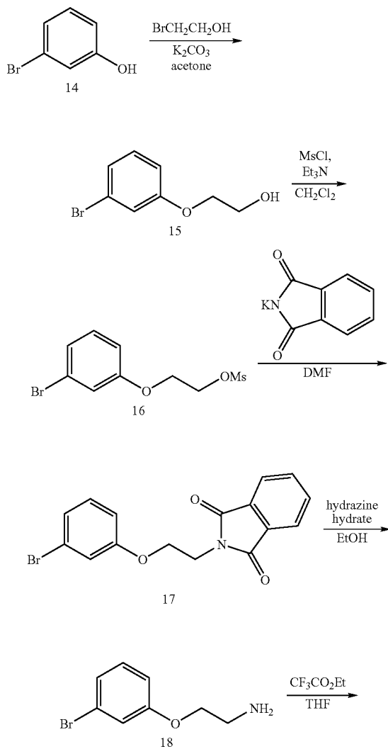
SCHEME 4
