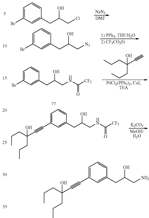
SCHEME 19
