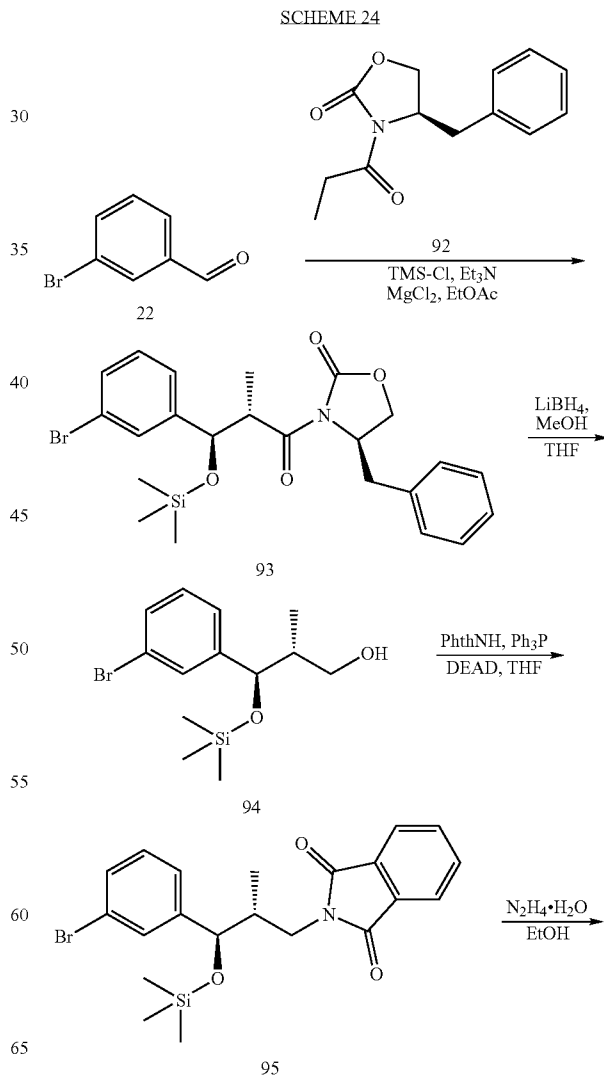
SCHEME 24
