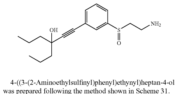
SCHEME 31
