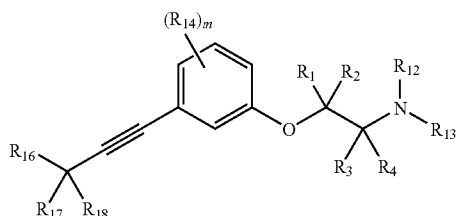
Formula (IIIb)
