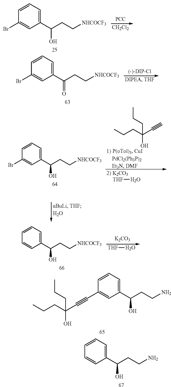
Scheme 16
