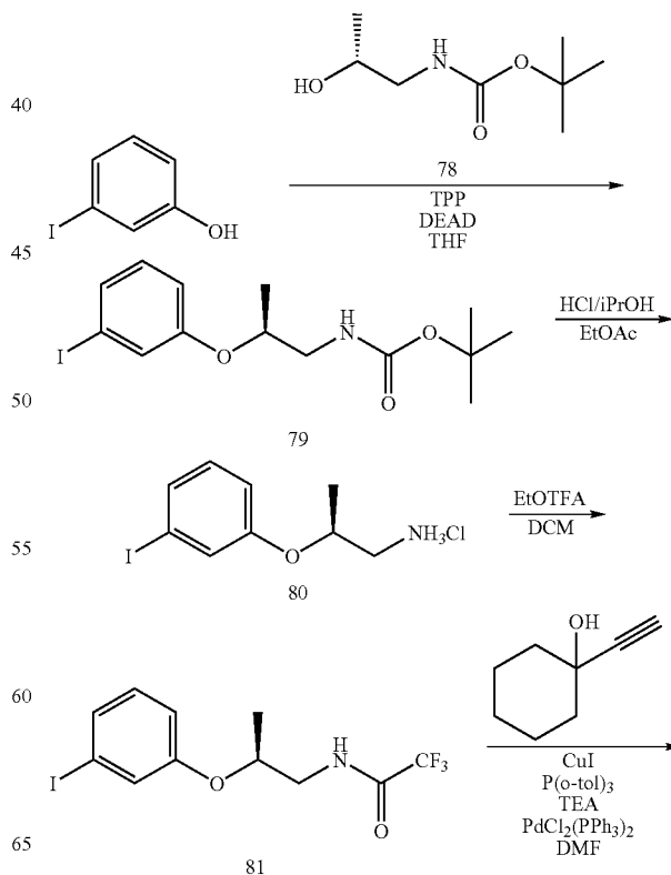
SCHEME 20
