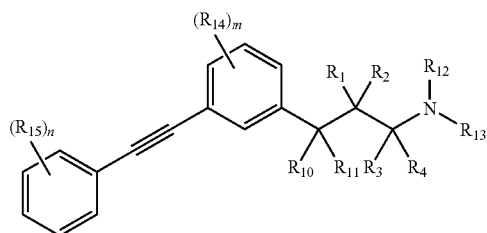
Formula (IIb)
