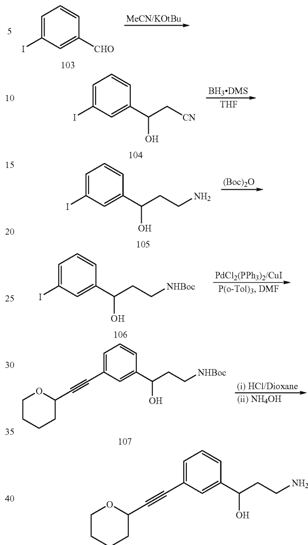
SCHEME 26
