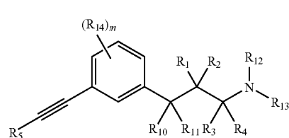
Formula (II)
