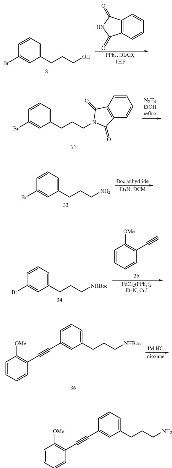
SCHEME 7
