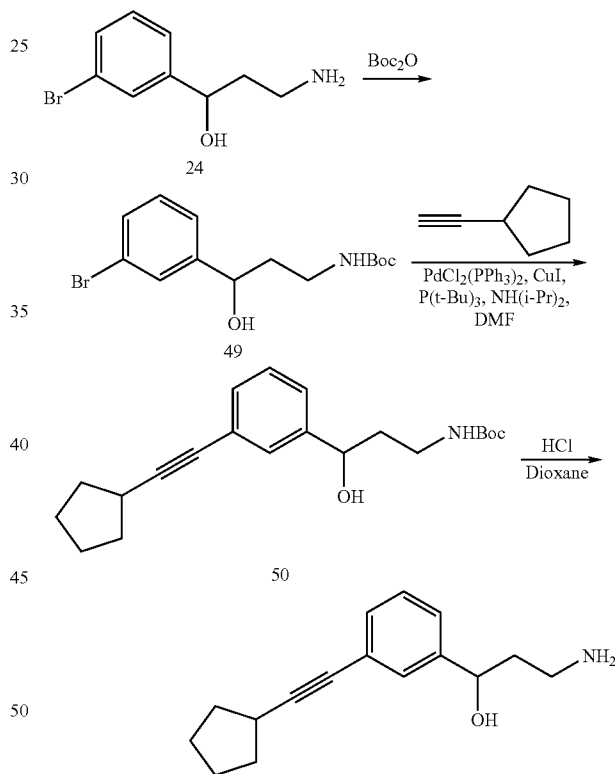
SCHEME 10
