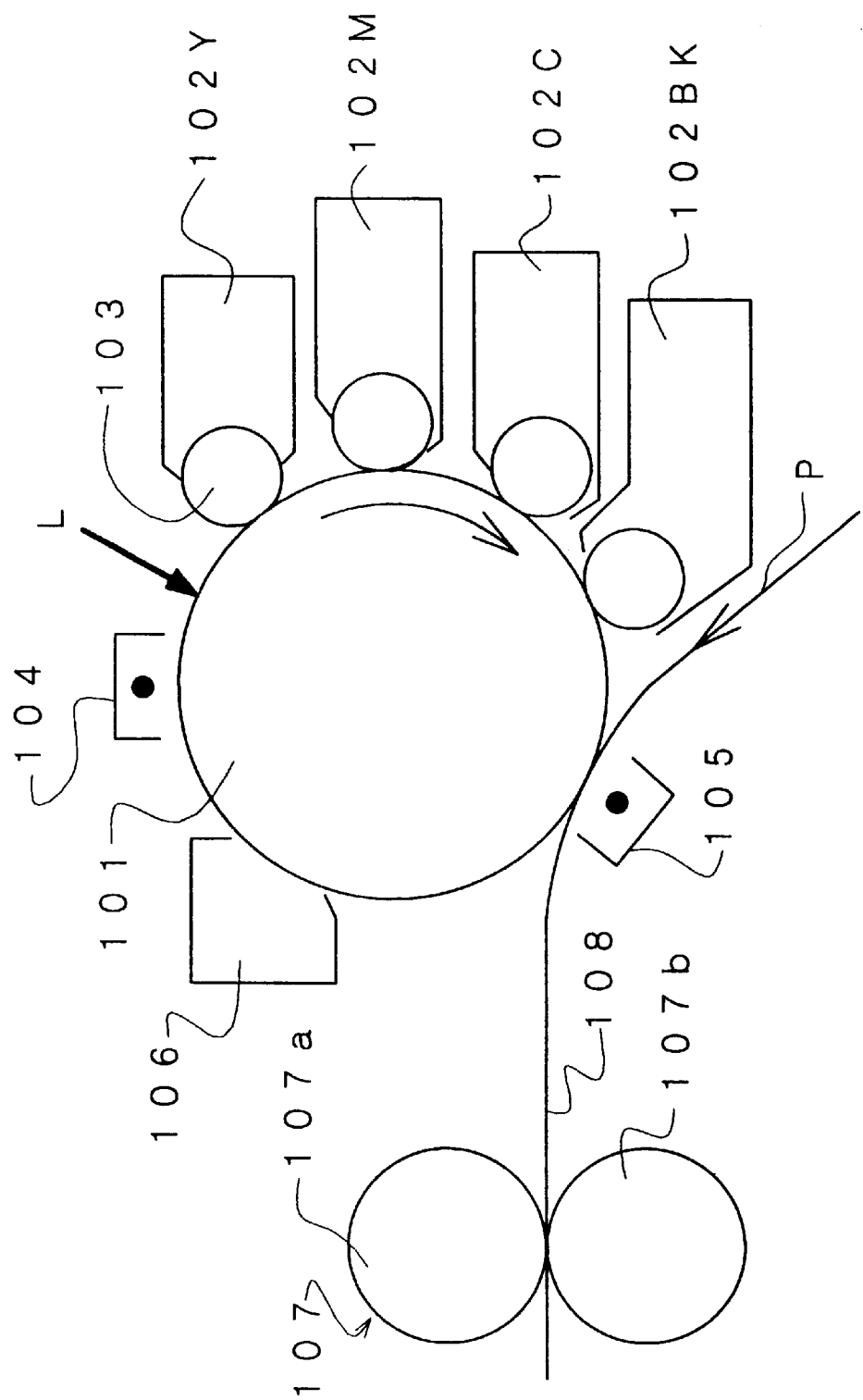
FIG. 6 (PRIOR ART)
