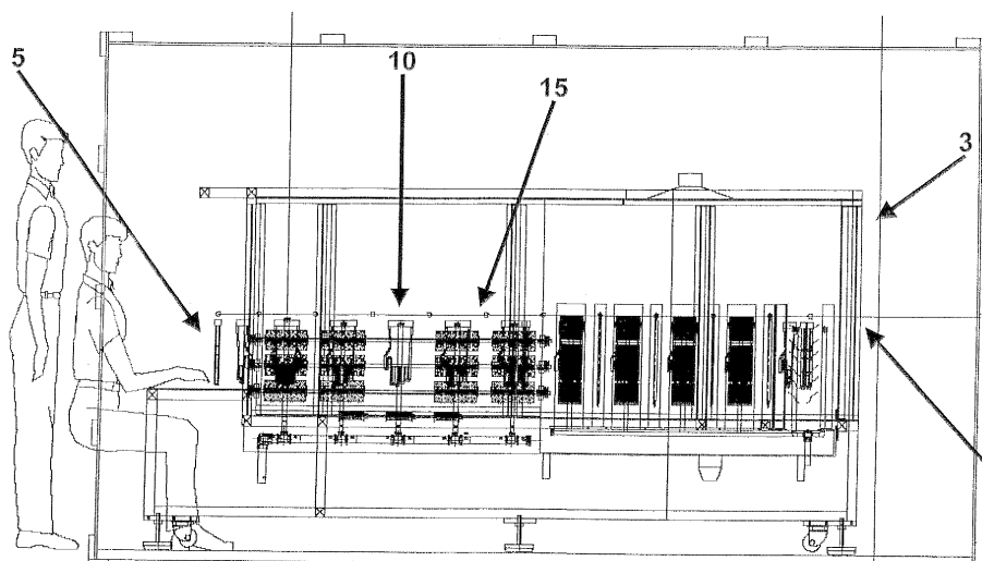
Figure 1: Glove reprocessing unit, Elevation view
