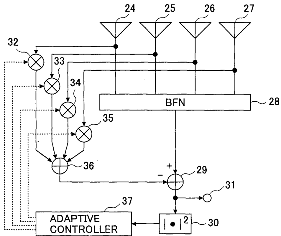
FIG.2 PRIOR ART
