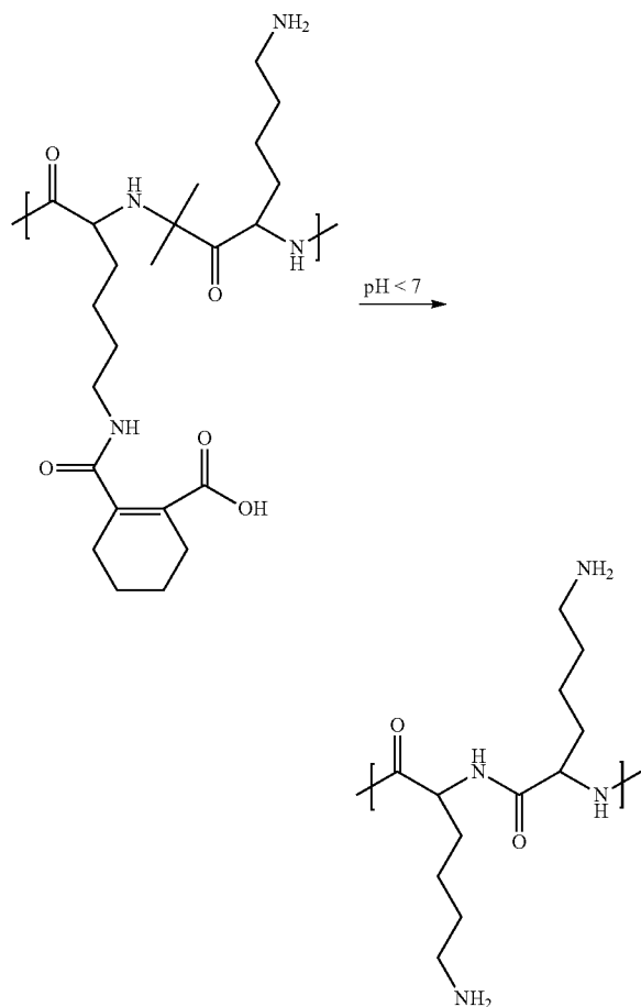
Scheme 7: Charge-reversal polylysine
