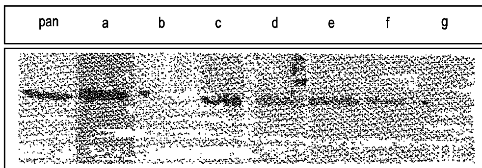
PEPTIDE COMPETITION FOR ANTI-Rb [pT821]
