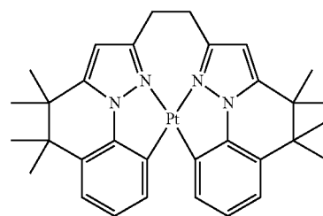
Compound Pt31
