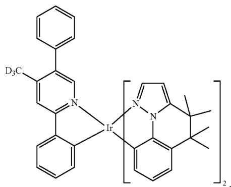
Compound Ir891
