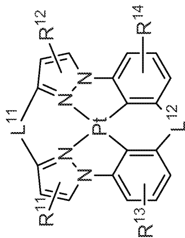
Formula III
