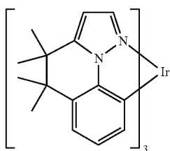
Compound Ir1
