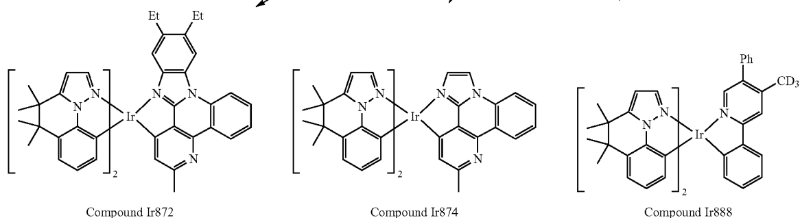
Compound Ir872
