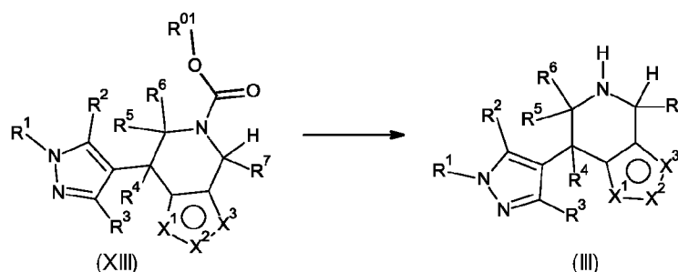
Scheme 8
