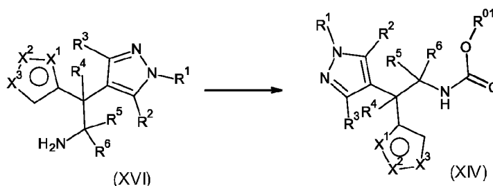
Scheme 10
