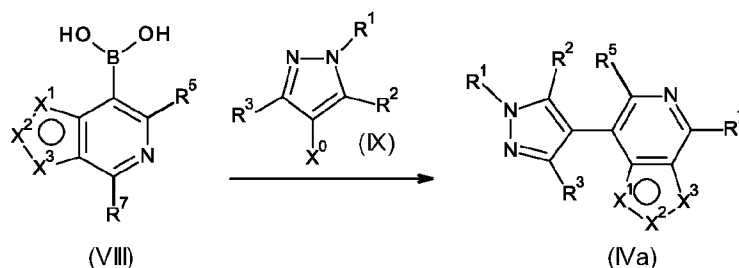
Scheme 5
