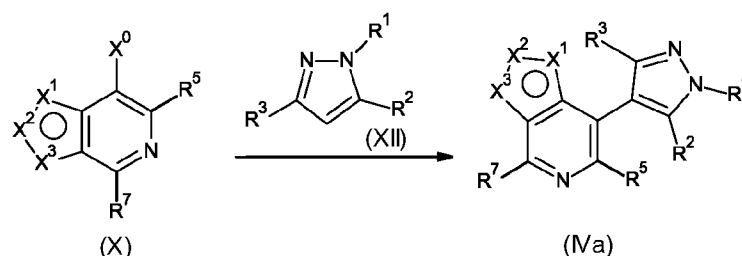
Scheme 7
