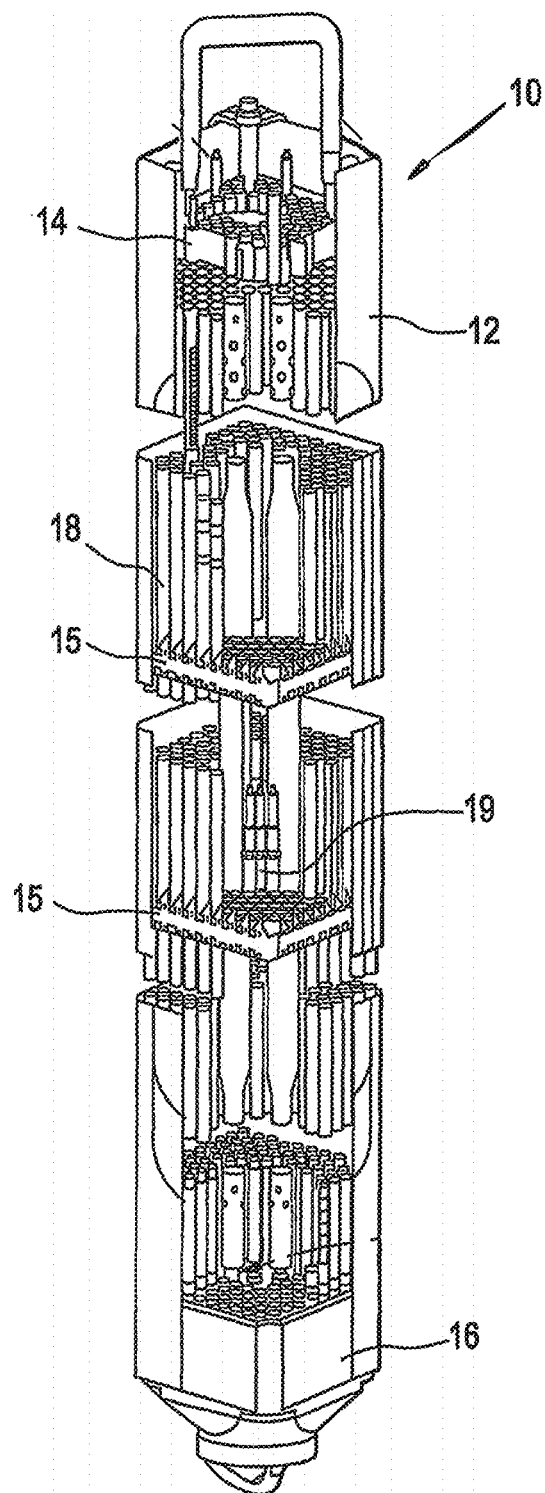
FIG. 1 CONVENTIONAL ART
