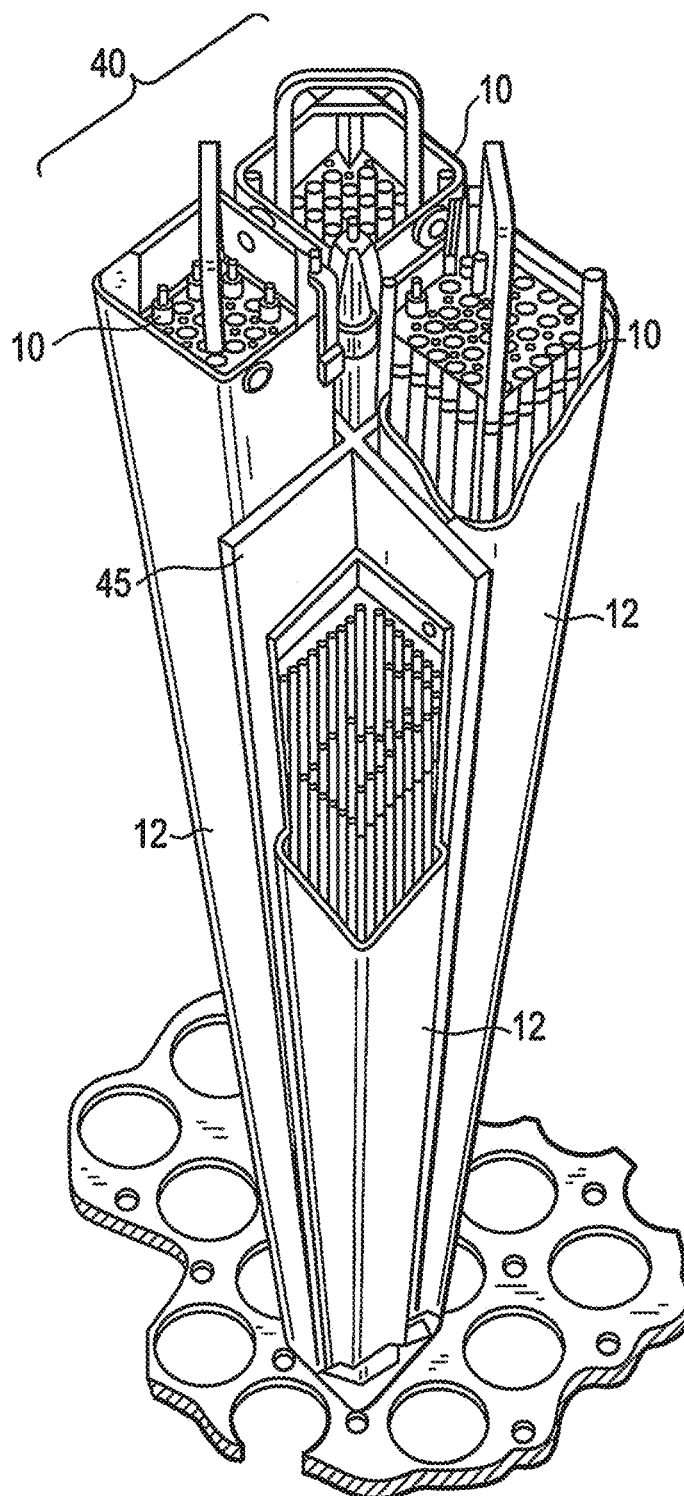
FIG. 2 CONVENTIONAL ART
