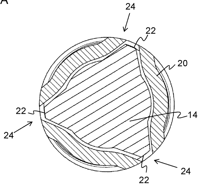
FIGURE 11 Section B-B
