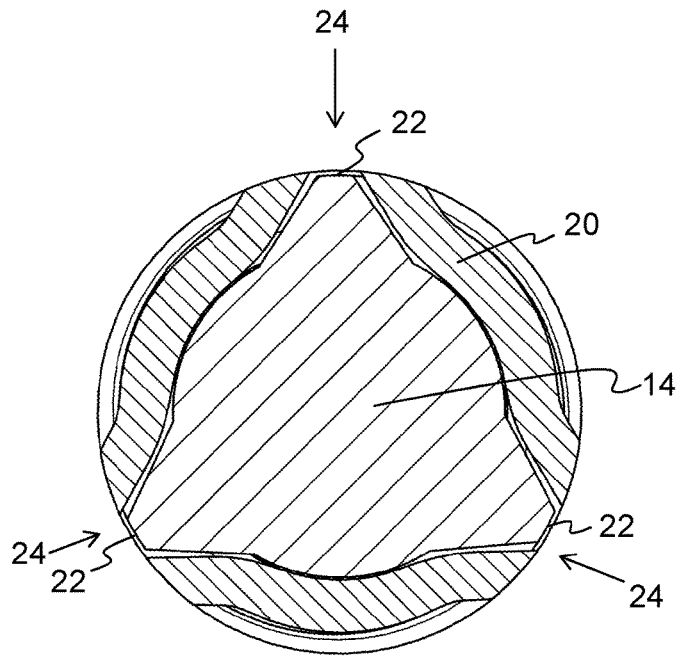
FIGURE 8 Section A-A
