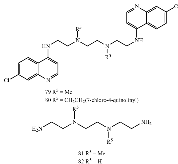
Scheme 10
