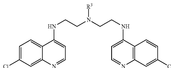
Scheme 8
