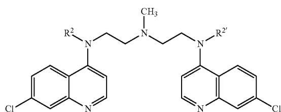
Scheme 7
