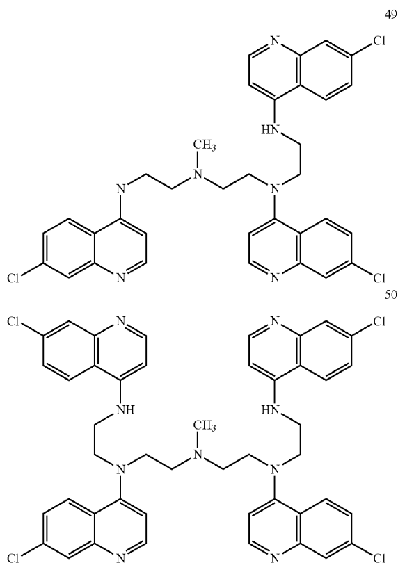
Scheme 6
