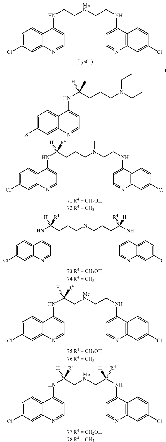
Scheme 9
