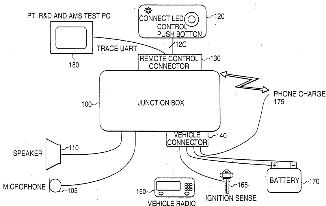
FIG. 1 REMOTE CONTROL
