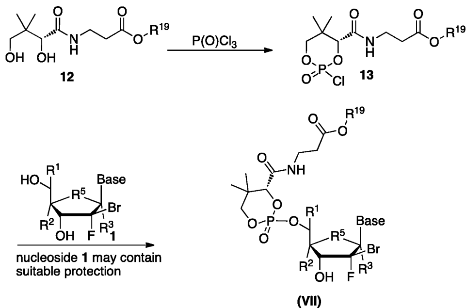
Scheme 34 A synthetic approach to monophosphate prodrugs VII . (Base, R^1 , R^2 , R^3 , R^5 and R^{19} are as defined in active compound section).
