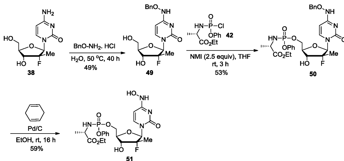
Scheme 19. Synthesis of N 4 -hydroxycytidine 2'-deoxy-2'- \alpha -fluoro-2'- \beta - C -Me nucleoside prodrug 51
