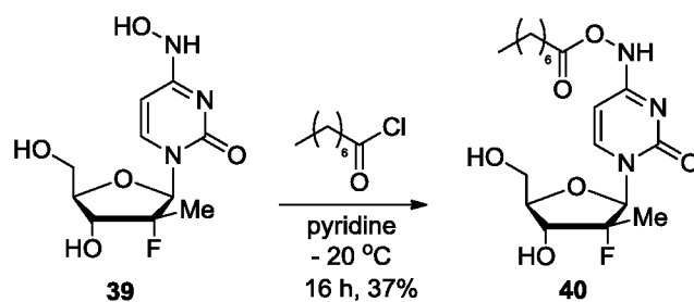
Scheme 16. Synthesis of N 4 -(Octanoyloxy)cytidine 2'-deoxy-2'-α-fluoro-2'-β-C-Me nucleoside 40
