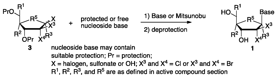
Scheme 28 An alternate synthetic approach to nucleosides 1 . (Base is defined in active compound section)
