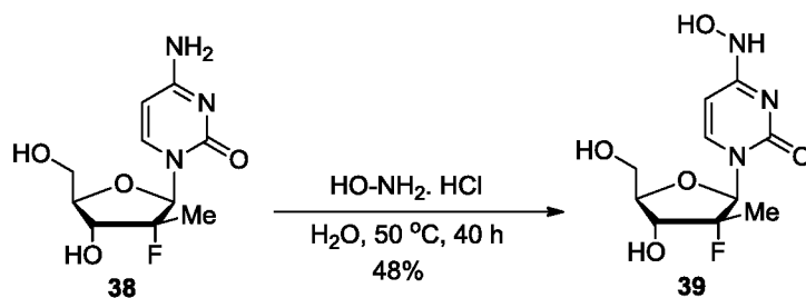
Scheme 15. Synthesis of N^4 -hydroxycytidine 2'-deoxy-2'- \alpha -fluoro-2'- \beta -C-Me nucleoside 39
