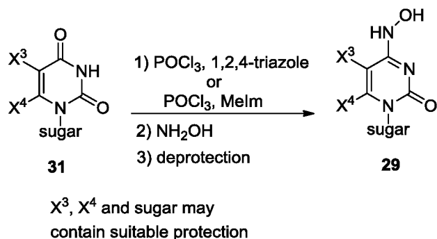
Scheme 12 An alternate synthetic approach to nucleosides 29 . ( \text{X}^3 , \text{X}^4 , \text{R}^1 and sugar are as defined in active compound section)
