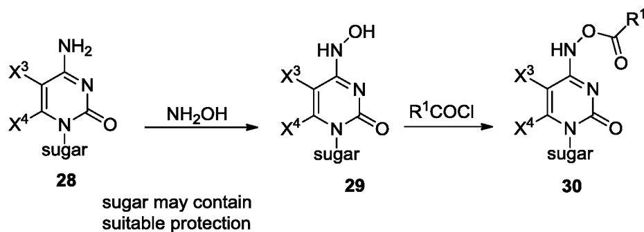
Scheme 11 Synthetic approach to nucleosides 29 and 30 . ( \text{X}^3 , \text{X}^4 , \text{R}^1 and sugar are as defined in active compound section)
