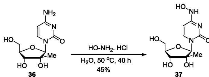
Scheme 14. Synthesis of N^4 -hydroxycytidine 2'-C-Me nucleoside 37
