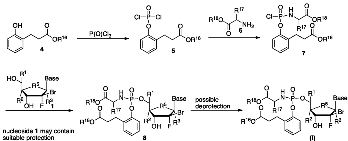
Scheme 32 A synthetic approach to monophosphate prodrugs I . (Base, R^1 , R^2 , R^3 , R^5 , R^{16} , R^{17} , and R^{18} are as defined in active compound section).
