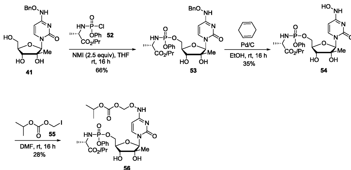
Scheme 19. Synthesis of N 4 -hydroxycytidine 2'-deoxy-2'- \alpha -fluoro-2'- \beta - C -Me nucleoside prodrug 51
