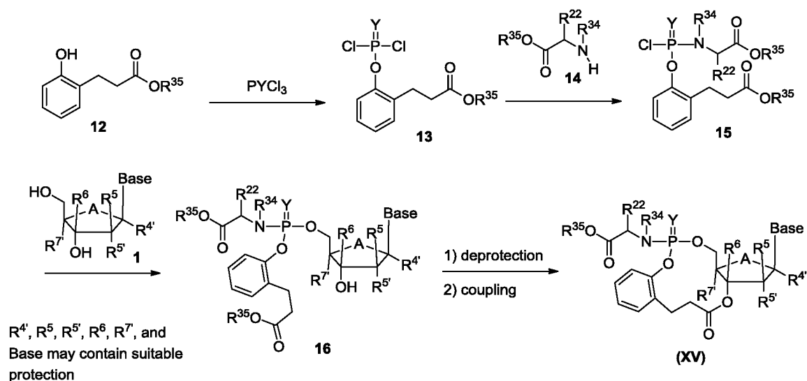
Scheme 3 A synthetic approach to monophosphate prodrug XXIII . (Base is a natural or unnatural nucleoside base; \text{R}^4 , \text{R}^5 , \text{R}^6 , \text{R}^7 , \text{Y} , \text{R}^{34} , \text{R}^{35} , \text{R}^{22} , and \text{R}^{7'} are as defined in active compound section)
