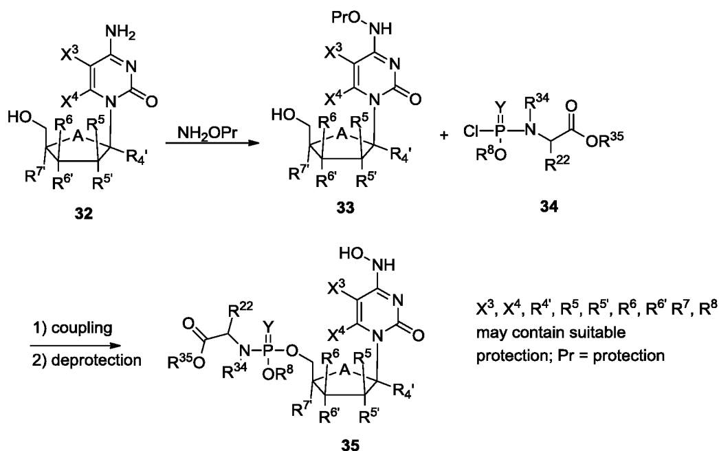
Scheme 13 Approach to monoposphate prodrug 35 . ( X^3, X^4, Y, R^{4'}, R^5, R^{5'}, R^6, Y, R^{34}, R^{35}, R^{22} , and R^{7'} are as defined in active compound section)
