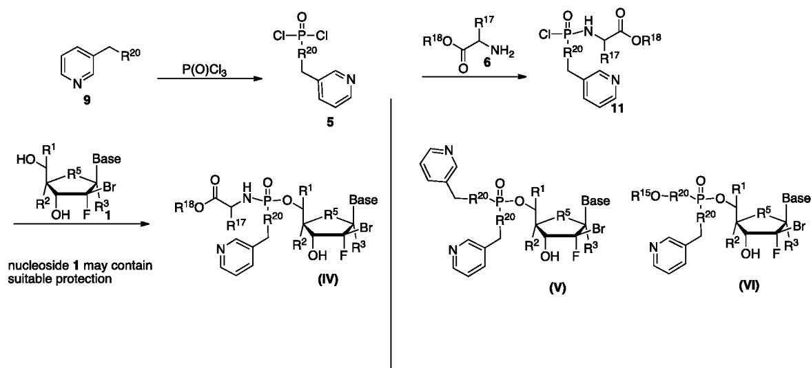
Scheme 33 A synthetic approach to monophosphate prodrugs IV-VI . (Base, R^1 , R^2 , R^3 , R^5 , R^{16} , R^{17} , and R^{18} are as defined in active compound section).
