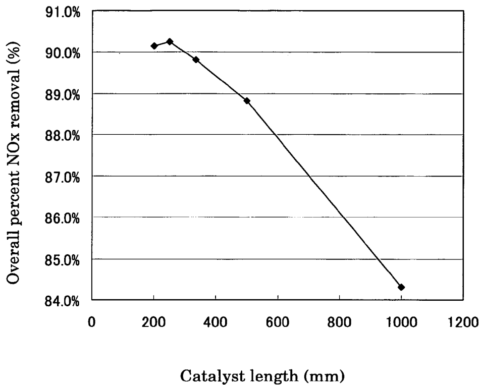
Catalyst length and performance in high-level NOx removal
