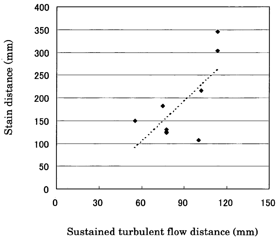
Sustained turbulent flow distance and catalyst stain distance
