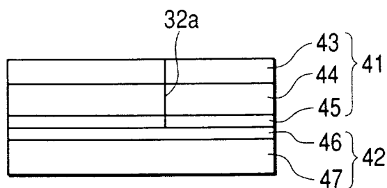
FIG. 16 PRIOR ART
