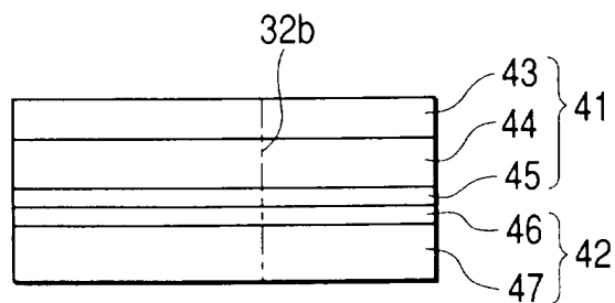
FIG. 17 PRIOR ART
