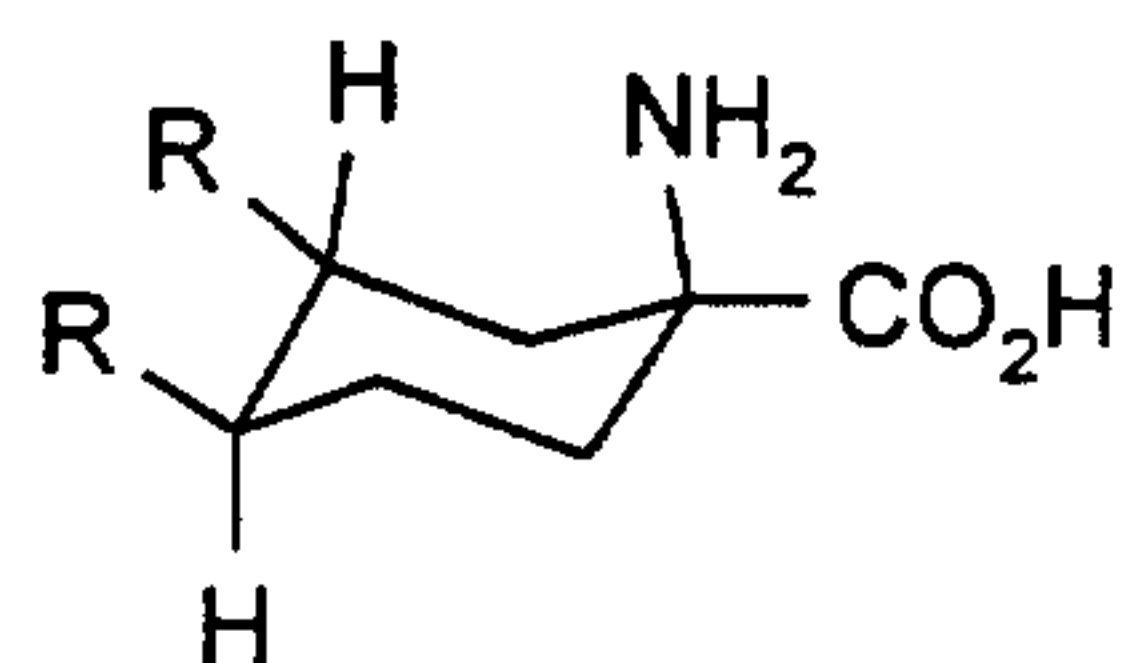
Bucherer-Bergs synthesis ( \beta isomer)
