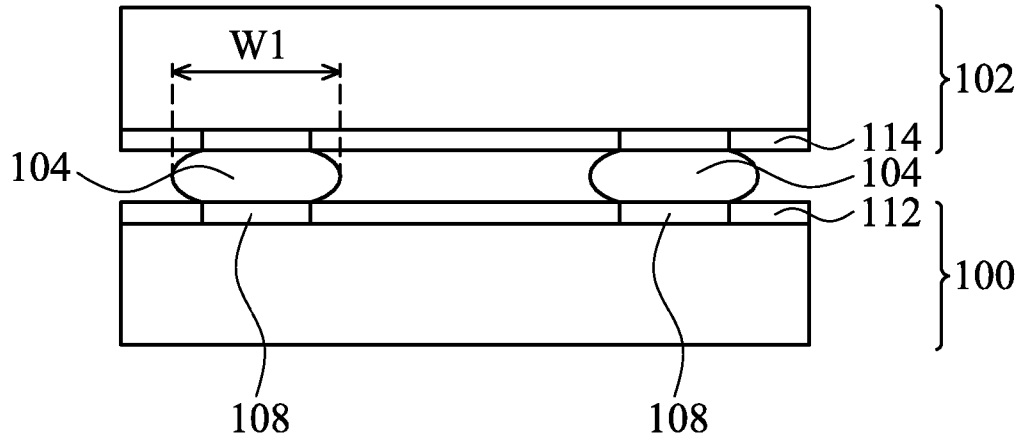
Fig. 3 ( Prior Art )
