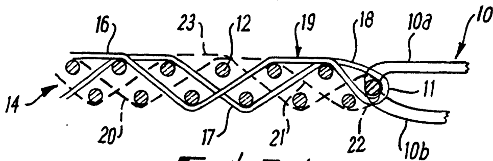
Fig. 1 (Prior Art)
