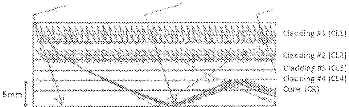
Figure 9(b2) 2D cross-section showing another exemplary design with ray tracing of a planar light concentrator consisting of multiple layers of polymers in a specific interfacial geometry with respect to each other and utilizing the effects of near-TIR, near-normal incidence, refraction and TIR.
