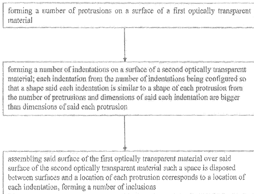
Figure 11(c). Fabrication method
