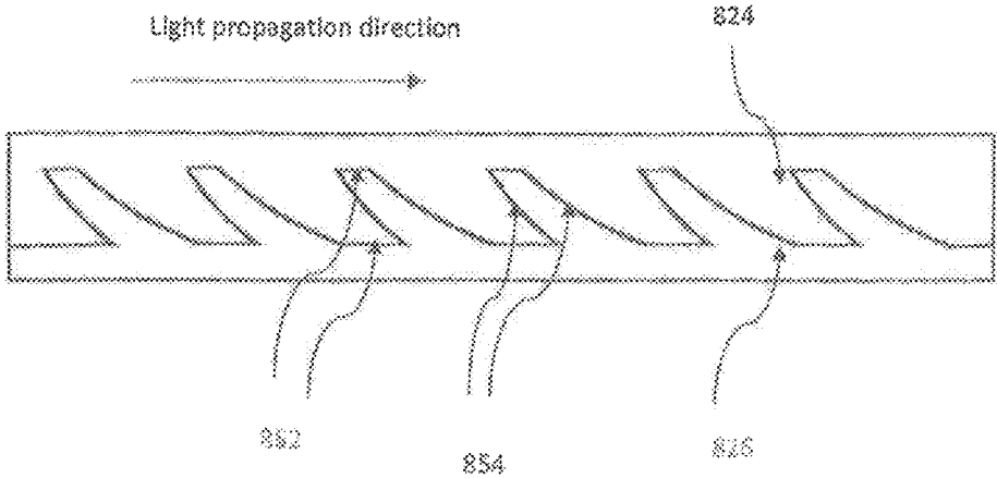
Figure 8(e4). Cross-section of the planar core layer with prismatic hetero-interface similar to Figure 8(e) but the interfacial structure in cross-section consisting of repetitions of flat sections and curved surfaces.
