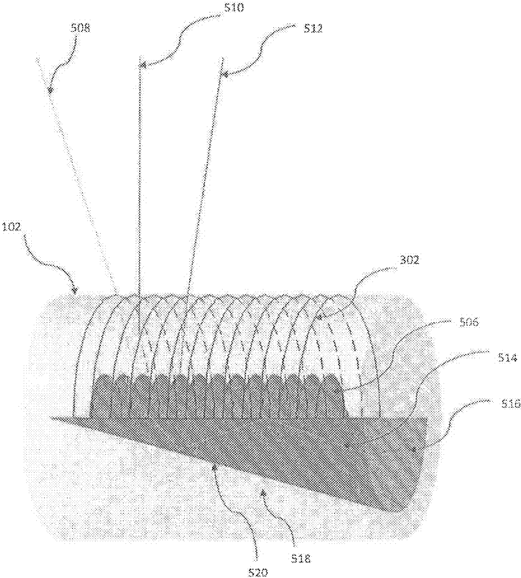
Figure 5: Ray traces of light going through the super-cladding, cladding and the core
