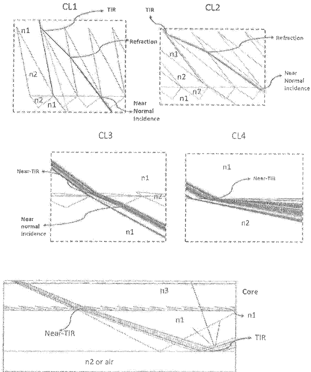
Figure 9(b3) Details of ray traces various layers (CL1, CL2, CL3, CL4 and Core) in the exemplary design shown in Figure 9(b2)
