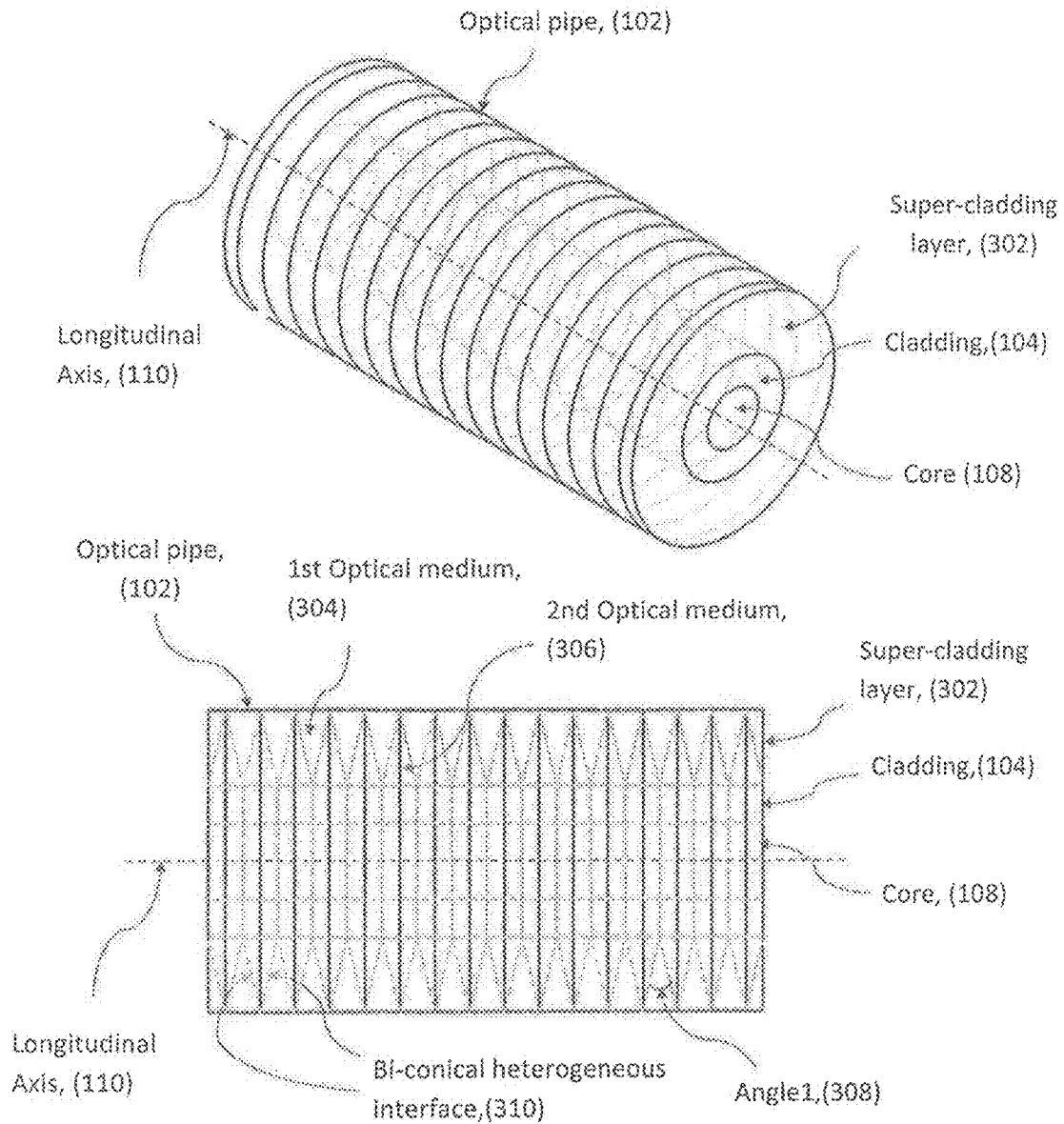
Figure 3. Super-cladding layer
