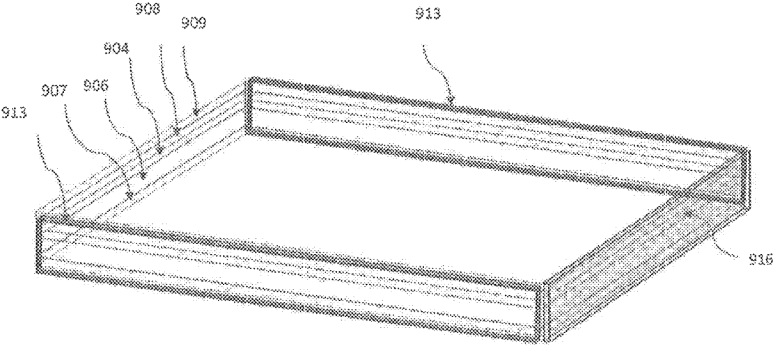
Figure 9(a1): Alternate construction of the planar light concentrator showing the various layers along with two side edges being mirrored and array of packaged solar cells on one edge.
