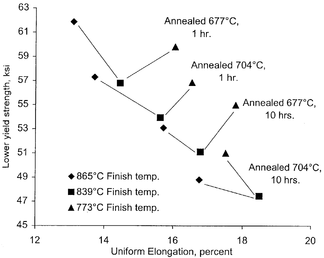
Figure 2. Laboratory Heats, Hot Rolled at Various Finishing Temperatures, after Various Sub-Critical Anneals
