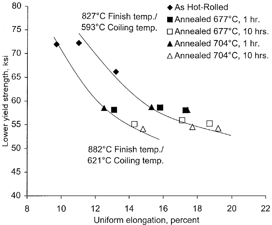
Figure 1. Samples from Commercially Hot-Rolled Coils -- As Hot Rolled and After Various Sub-Critical Anneals
