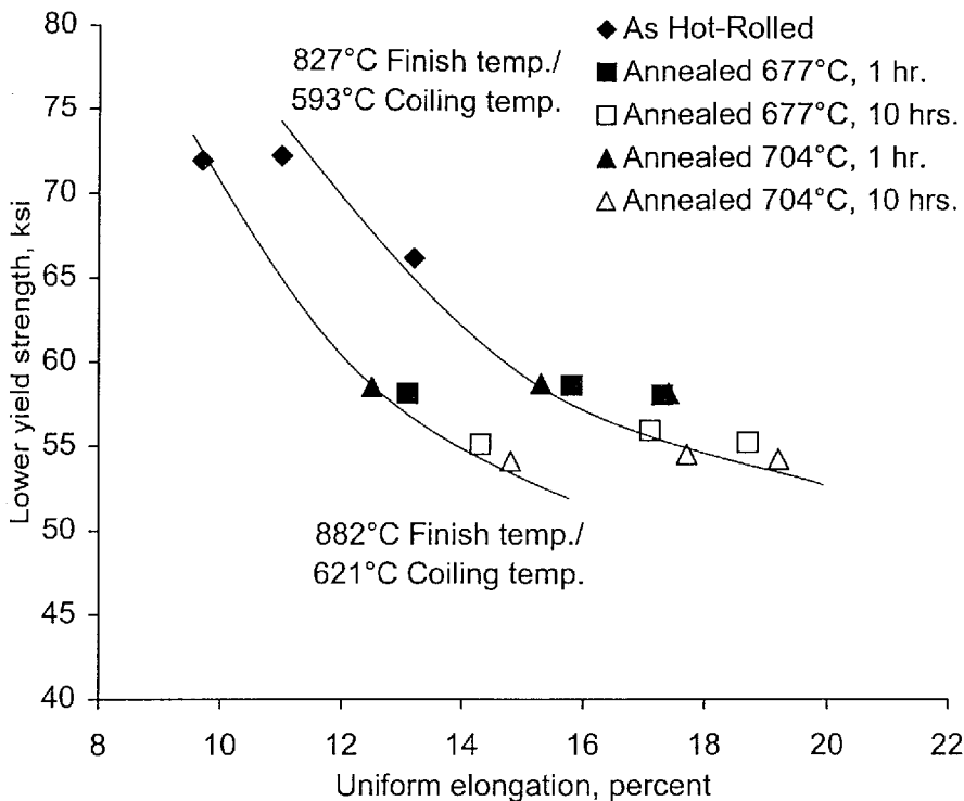
Samples from Commercially Hot-Rolled Coils -- As Hot Rolled and After Various Sub-Critical Anneals
