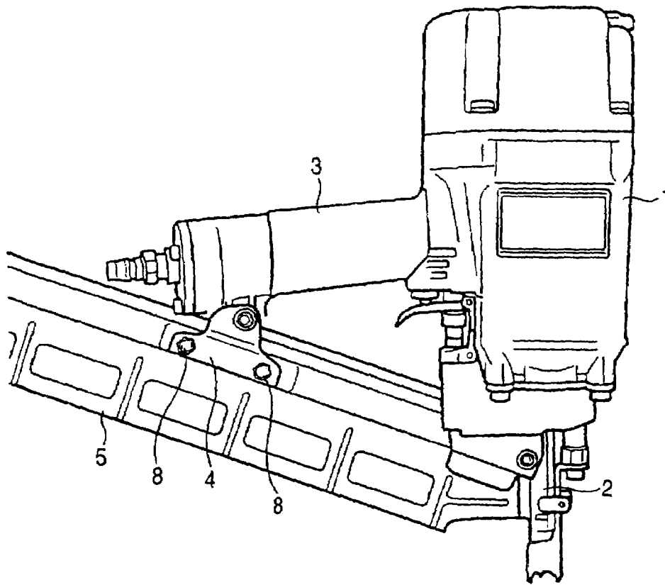
FIG. 4 PRIOR ART
