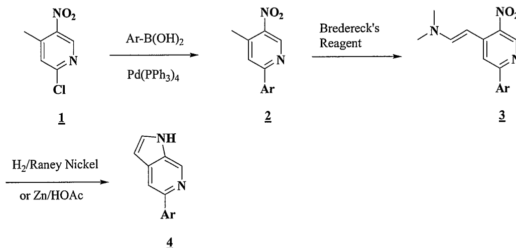
Scheme 1. Preparation of Intermediate 4 for synthesis of compounds of Formula Ia.
