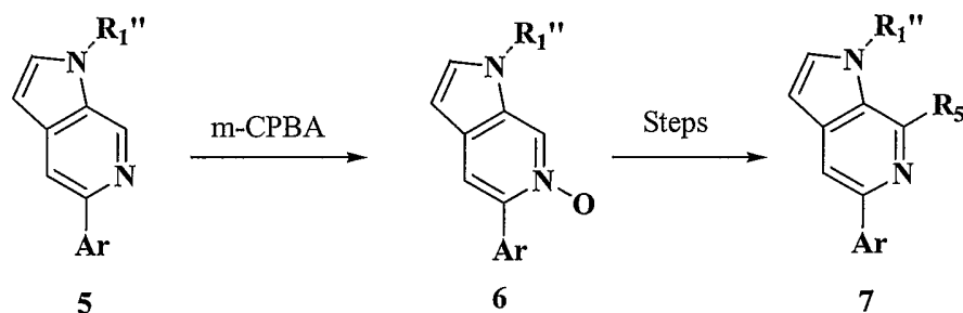
Scheme 3. Preparation of Compounds of Formula Ia wherein R 5 is attached to Compound 5.
