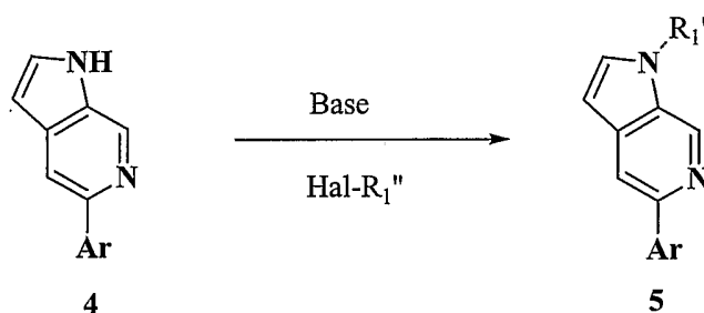
Scheme 2. Preparation of compounds of Formula Ia wherein R_1'' is attached to intermediate 4.
