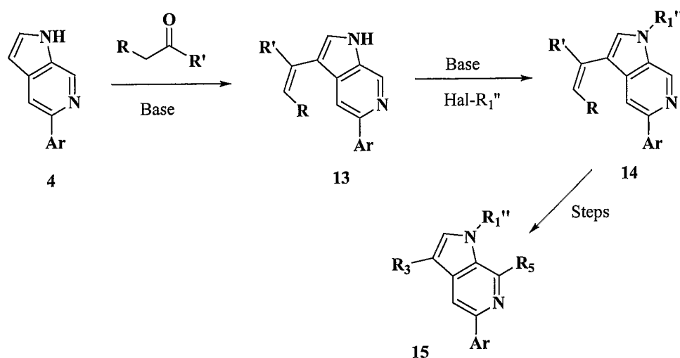
Scheme 6 Preparation of compounds of Formula I or Formula II.
