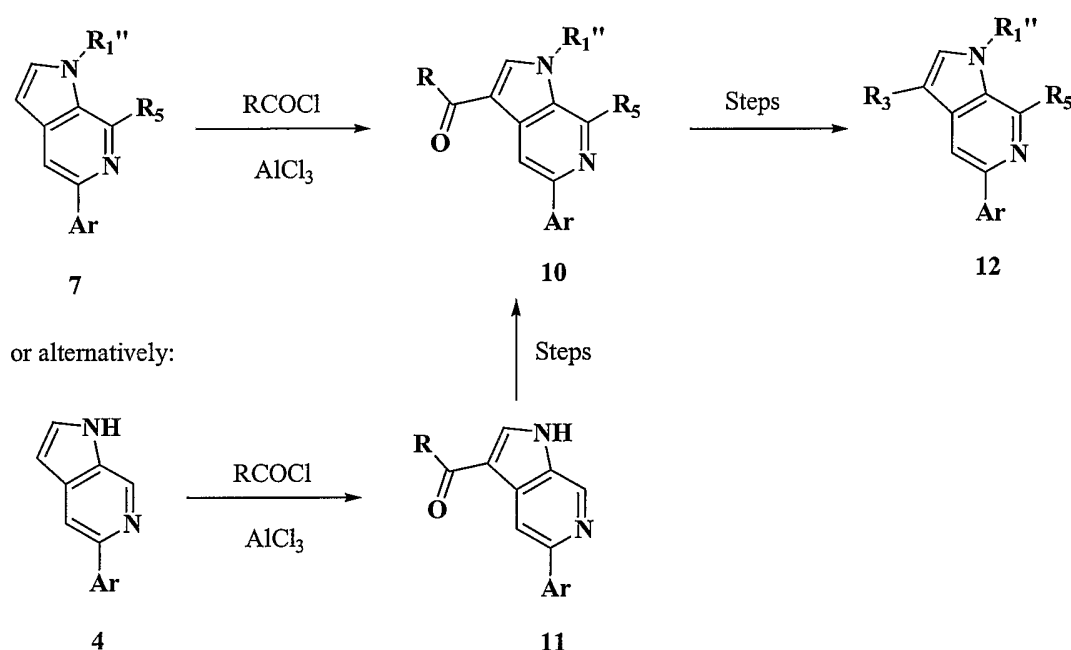
10 Scheme 5. Preparation of compounds of Formula I or Formula II.
