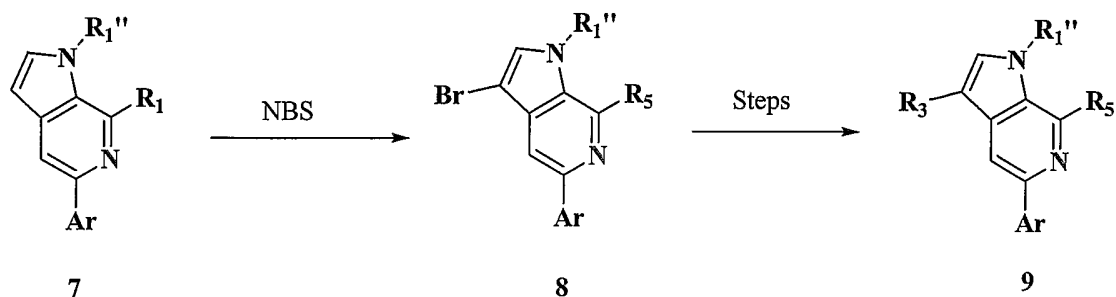
Scheme 4. Preparation of compounds of Formula I or Formula II where R 3 is introduced.
