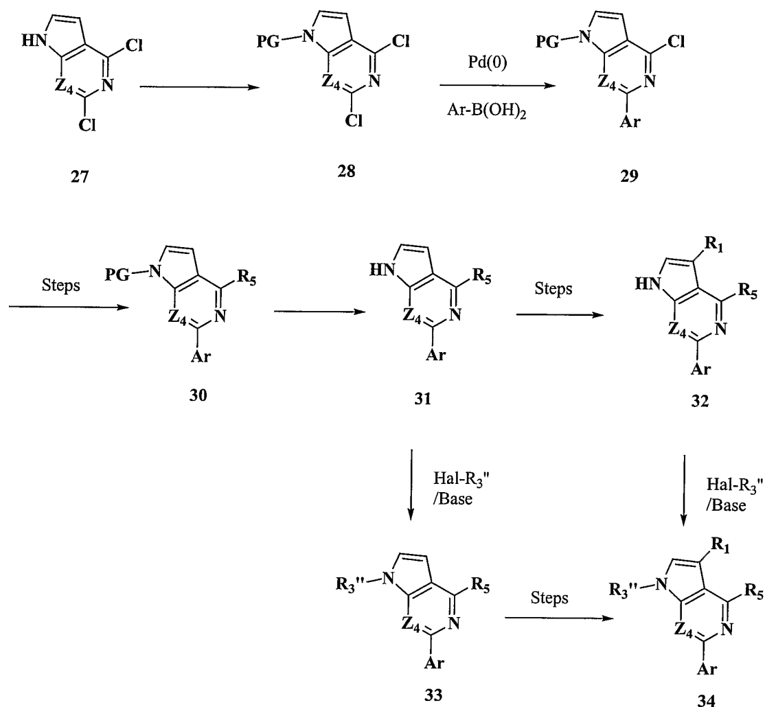
Scheme 9 Preparation of compounds of Formula I or Formula II in which Z_1 is CR_1 and Z_3 is NR_3'' .
