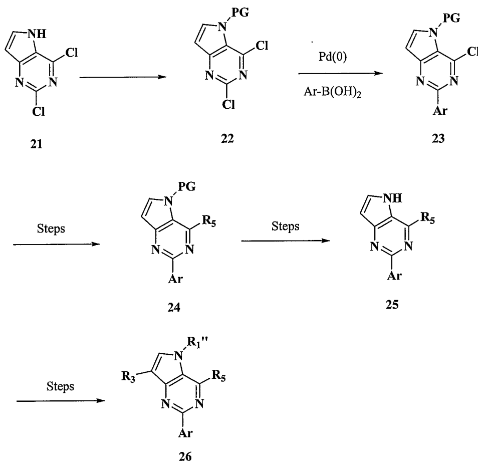
Scheme 8 Preparation of compounds of Formula I or Formula II wherein Z_4=N .
